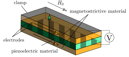
Fig. 4. Three layers magneto-electric heterostructure, the colored arrows represent the poling direction of the materials.
