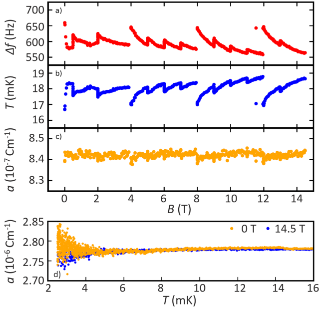
FIG. 4. a) The resonance width of ATF5 as function of applied magnetic field during a sequence of field sweeps. b) The temperature inferred from the melting curve thermometer during the same field sweeps. c) The tuning fork constant, a , as calculated from the fitted resonance curve as a function of the applied field. d) The tuning fork constant, a as a function of temperature for the CTF, during two different demagnetizations at 14.5 T (blue) and 0 T (orange)
