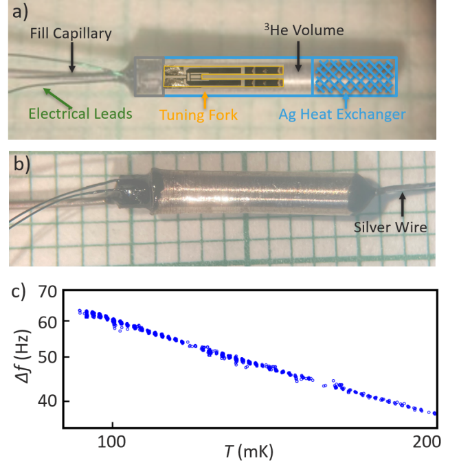
FIG. 5. Prototype tuning fork thermometers comprising a CTF and silver sinter heat exchanger encased in a silver tube. a) Schematic overlay showing the internal components and dimensions b) a newer prototype, showing the silver wire for the thermal link to the sample c) The resonance width as a function of temperature for the TFT pictured in b).
