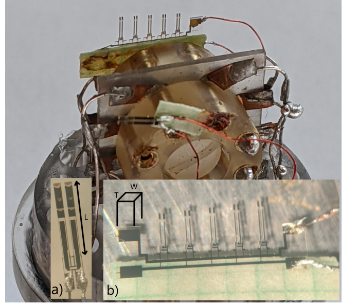
FIG. 1. The polycarbonate cell insert used in this work, showing the CTF (front) and Array of tuning forks (back). Inset: the tuning forks studied in this work. a) an Epson C-002RX commercial tuning fork (CTF), nominal resonance frequency 32.768 kHz. b) an array of 5 tuning forks, provided by Viktor Tsepelin, Lancaster University, UK 34 .
