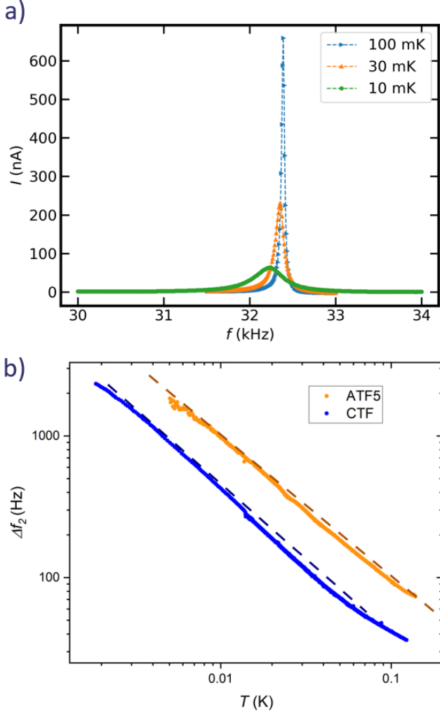
FIG. 2. a) Resonance curves (response current as a function of frequency) at constant driving force for the CTF b) Resonance width as a function of temperature for CTF and ATF5, the dashed lines are guides to the eye for T^{-1} .
