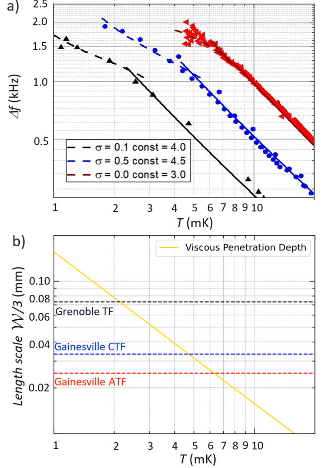
FIG. 3. a) The resonance width as a function of nuclear stage temperature for GTF(Black) CTF(Blue) and ATF5(red). The solid lines are calculated values of the width using hydrodynamic functions from Brumley et al 31 , the dashed lines are a slip correction 32 where the specularity, \sigma , and slip length coefficient const are fit parameters. b) A plot showing the tuning fork length scale versus temperature. The solid line shows the viscous penetration depth, and the dotted lines the values of W/3 for each tuning fork measured here.
