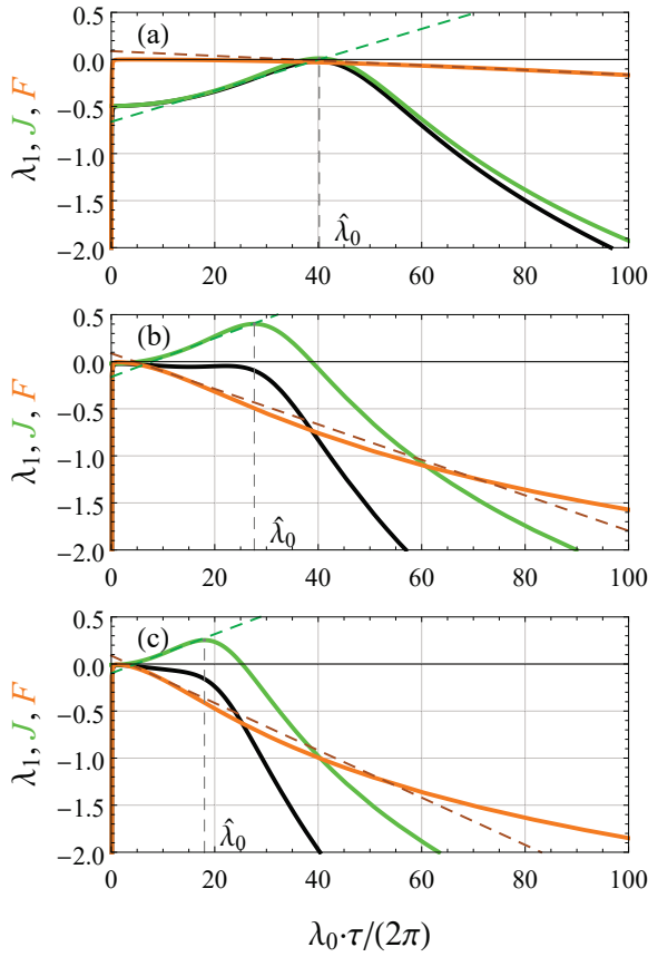
FIG. 3. Decomposition of a PC spectrum real part \lambda_1 (black line) into the part J defining a modulational instability caused by the relaxation oscillations undamping (green line, Eq. (8)) and the part F accounting for filtering (orange line, Eq. (9)). The dashed grey line shows the position of the J function maximum at \hat{\lambda}_0 . The dashed green (orange) line shows a slope of a curve J ( F ) at the point \hat{\lambda}_0/2 ( 1/(2\tau_L) ) for illustrative purposes. The parameters are: (a) P = 0.4 , \eta = 0.61 , \tau_L = 1 ; (b) P = 0.2 , \eta = 0.98 , \tau_L = 7.5 ; (c) P = 0.1 , \eta = 0.99 , \tau_L = 10 . The other parameters are given in the text.
