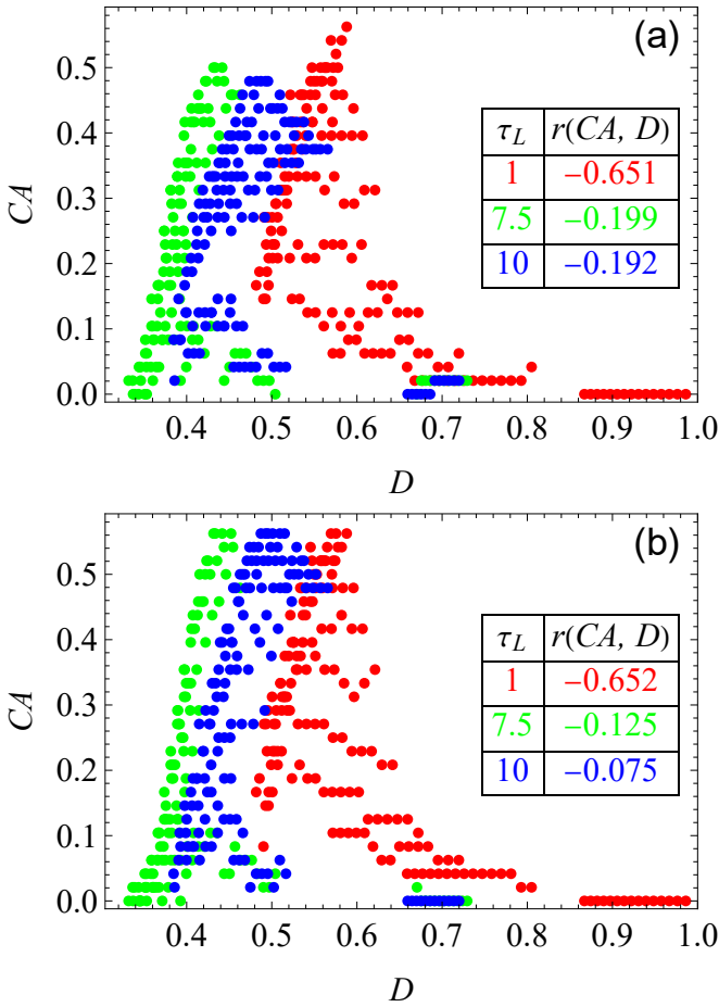
FIG. 13. The correlation scatter plots CA vs. D for negative (a) and positive (b) feedbacks. The color corresponds to a value of the low-pass filtering parameter: \tau_L = 1 (red); \tau_L = 7.5 (green); \tau_L = 10 (blue). The Pearson correlation coefficient values r are given in the insets.
