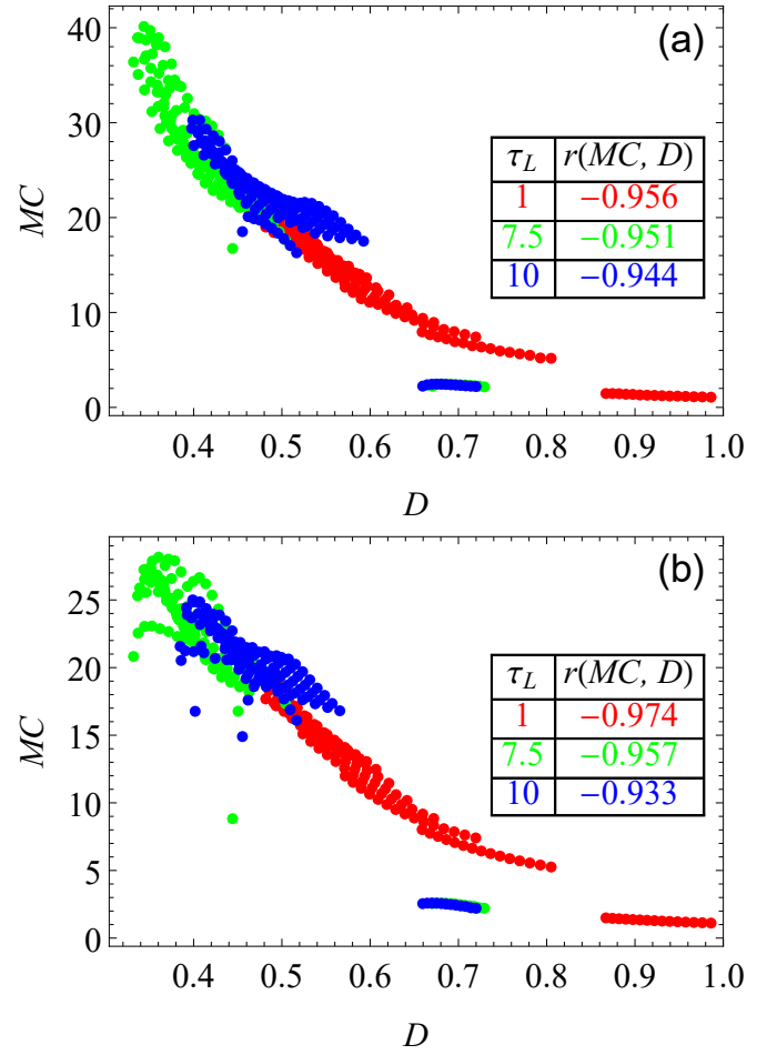
FIG. 8. The correlation scatter plots MC vs. D for negative (a) and positive (b) feedback signs. The color corresponds to a value of the low-pass filtering parameter: \tau_L = 1 (red); \tau_L = 7.5 (green); \tau_L = 10 (blue). The Pearson correlation coefficient values r are given in the insets.
