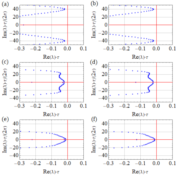
FIG. 2. Eigenvalue spectra, from top row to bottom: (a,b) \tau_L = 1 ; (c,d) \tau_L = 7.5 ; (e,f) \tau_L = 10 . The values of \eta and P are such that for every \tau_L the system operates close to a Hopf bifurcation, and with maximal MC : (a) P = 0.4 , \eta = -0.61 ; (b) P = 0.4 , \eta = 0.61 ; (c) P = 0.2 , \eta = -0.98 ; (d) P = 0.2 , \eta = 0.98 ; (e) P = 0.1 , \eta = -0.99 ; (f) P = 0.1 , \eta = 0.99 . The other parameters are given in the text.
