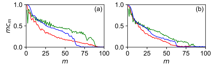
FIG. 9. The memory curve for negative (a) and positive (b) feedback: m is the number of delayed input steps for \tau_L = 1 (red); \tau_L = 7.5 (green); \tau_L = 10 (blue). The other parameters are the same as in Fig. 2.
