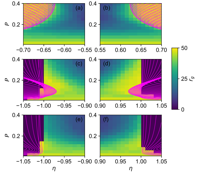
FIG. 11. 2D maps of the system's generalization rank, from top row to bottom: (a,b) \tau_L = 1 ; (c,d) \tau_L = 7.5 ; (e,f) \tau_L = 10 . The other parameters are given in the text.
