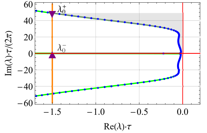
FIG. 4. Graphical representation of the average distance D defined by Eq. 11. The green line is the PC spectrum given by Eq. 7, where \lambda_1 = \text{Re}(\lambda)\tau , which approximates the numerical eigenvalues (blue dots) very well. Orange line is \text{Re}(\lambda)\tau = -1.5 . Purple triangles denote the points at the PC spectrum corresponding to \lambda_0^- and \lambda_0^+ defining the averaging interval where \lambda_1 \geq -1.5 . The grey shaded area corresponds to the integral in Eq. 11. The parameters are the same as in Fig. 2(c).
