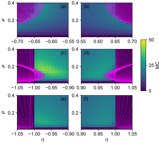
FIG. 7. 2D maps of the system's memory capacity, from top row to bottom: (a,b) \tau_L = 1 ; (c,d) \tau_L = 7.5 ; (e,f) \tau_L = 10 . The magenta lines are the Hopf bifurcation borders. The other parameters are given in the text.
