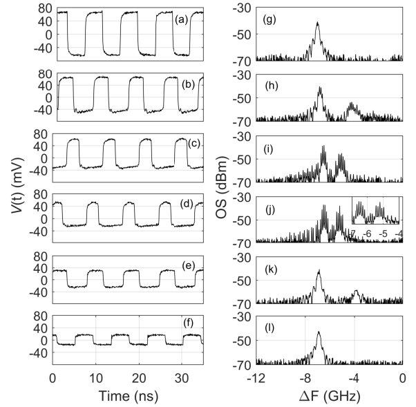
FIG. 2. PD output voltage V(t) tracking the time-dependent AC component of optical intensity I(t) (left-column) and corresponding optical spectra (right-column) for J = 48.40 mA as \eta is ramped down (a) 0.97, (b) 0.88, (c) 0.75, (d) 0.59, (e) 0.41, (f) 0.30 with f_{rep} = 4\tau^{-1} . Note the appearance of doublets only for intermediate values of \eta with J held fixed. The inset in (j) shows evidence of the SW repetition rate f_{rep} in the spacing of the small peaks underlying the doublet. Note that the duty cycle is close to 50% in (a) and (l).
