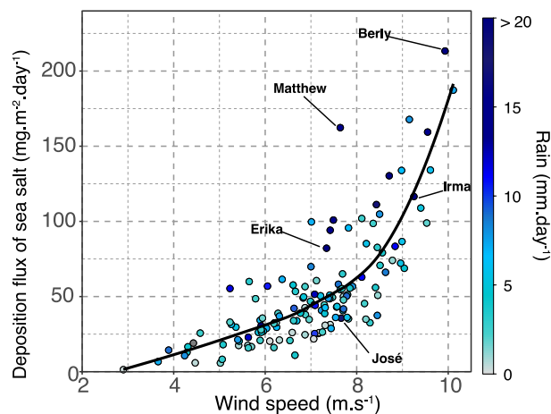
Figure 4. Sea salt deposition fluxes as a function of the averaged wind speed showing the daily precipitation rate levels ( \text{mm}\cdot\text{day}^{-1} ), with the name of the five cyclone events occurring during the sampling period. The smooth correlation curve is obtained using the “ggplot2” R package with the “geom_smooth” function, to see the trend of the nonlinear relationship between two variables (R Core Team, 2021; Wickham, 2016). As the average daily rainfall ranges from 0 to 67\text{ mm}\cdot\text{day}^{-1} during the whole sampling period, and because only two samples correspond to a sampling period with average daily rainfall over 20\text{ mm}\cdot\text{day}^{-1} , all the samples corresponding to daily rainfall levels over 20\text{ mm}\cdot\text{day}^{-1} are shown in a dark blue color.
