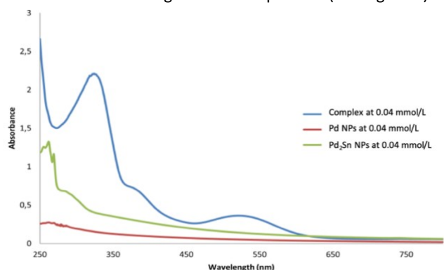
Figure 1 – UV-Visible absorption spectrum of Pd 2 (dba) 3 -dba, palladium, and palladium-tin colloids in THF with a Pd concentration of 40 μmol/L at 298 K.
