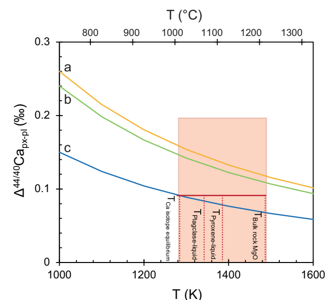
Figure 1 Plot of \Delta^{44/40}\text{Ca}_{\text{px-pl}} versus equilibrium temperature of minerals. The red square represents the range of fractionation between pyroxenes and plagioclases and the relative temperature of mineral differentiation. Three solid lines are theoretical equations of equilibrium fractionation between pyroxenes and plagioclase: a, diopside-labradorite (Antonelli et al. , 2019); b, diopside-anorthite (Zhang et al. , 2018); c, diopside-anorthite (Huang et al. , 2019). Four dashed lines represent equilibrium temperatures determined by different methods.
