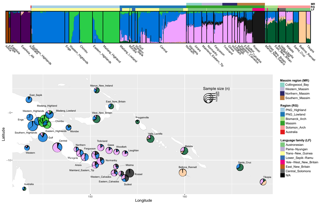
Fig. 2. ADMIXTURE analyses focusing on Oceanian structure. ADMIXTURE results for K = 8 (the optimal K with the lowest cross-validation error; supplementary fig. S8A, Supplementary Material online) on the top, plotted on a map at the bottom. Color bars on the top indicate the region (RG), language family (LF) for the Oceanian groups, and Massim region (MR) for the Massim groups. The size of the circle for each group on the map is proportional to the sample size.
