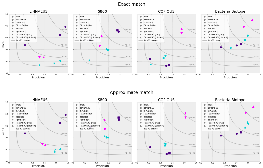
FIGURE 7 Precision and recall obtained on the four gold standard corpora using the exact match criterion (top) and the approximate match criterion (bottom). Grey lines represent iso- F_1 curves. The different colors are used to distinguish between the different categories of tools : dictionary-based NER systems (violet), scientific name taggers (blue) and deep neural networks (pink).
