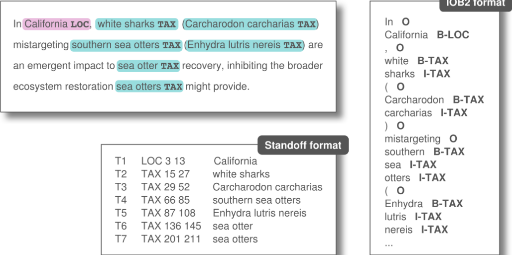
FIGURE 5 A gold standard corpus is a collection of manually annotated documents. An entity’s annotation includes at least the left and right boundaries of the entity span as well as its class. Standoff and IOB2 are the two most common tagging formats. In IOB2, the B- prefix indicates that the token is the beginning of an entity, and the I- prefix indicates that the token is inside an entity. An O tag indicates that a token belongs to no entity.
