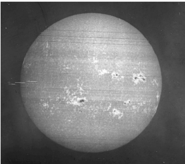
Spectroheliogram CaII K23 - 17 November 1893 Paris observatory
