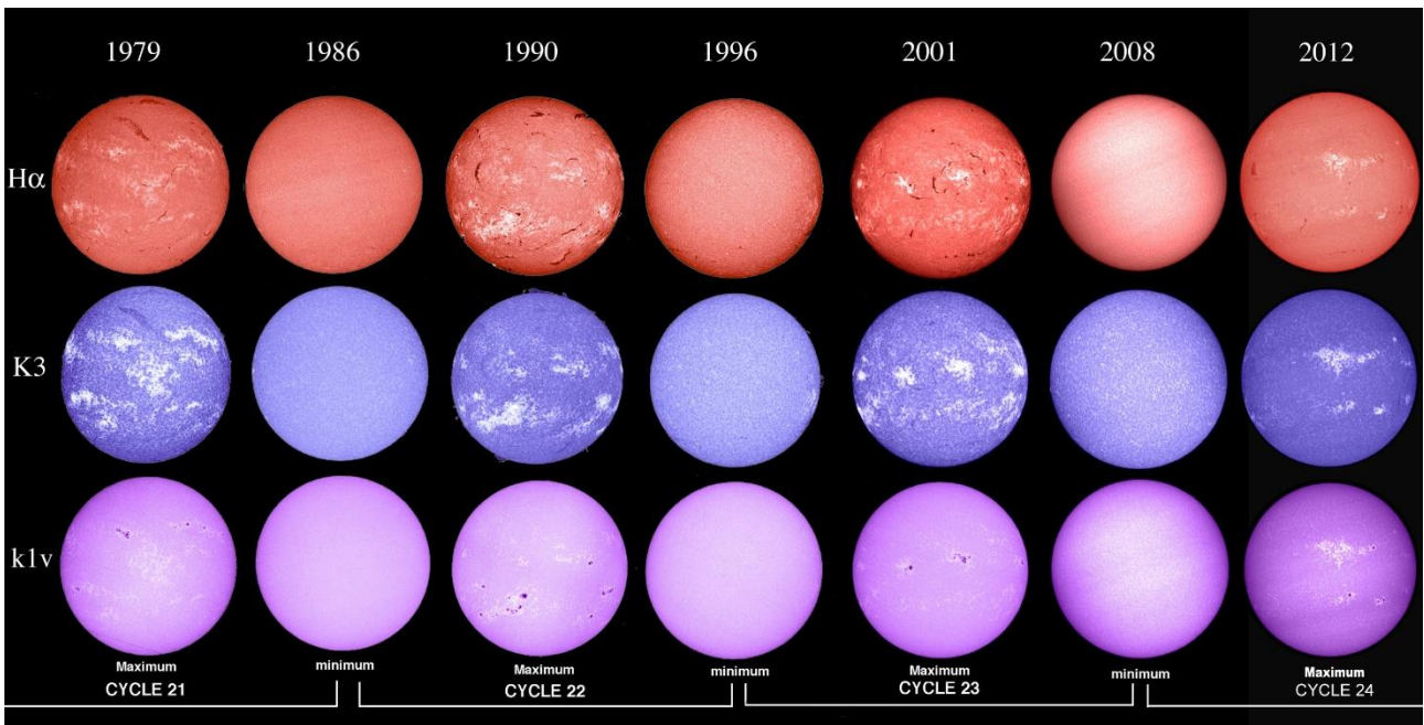
Figure 2. A subset of images at successive solar minima and maxima from Meudon spectroheliograph (the 11-year cycle). The chromosphere (with dark filaments and bright plagues) is observed in the centre of the H \alpha line or in the centre (K3) of the Call K line. The photosphere (sunspots and bright faculae) appears in the blue wing (K1v) of the Call K line. False colours. The various wavelengths reveal solar activity phenomena at different heights in the atmosphere. The structures are related to the solar magnetism, strong in sunspots, intermediate in facular regions and weak in filaments. Courtesy Paris observatory.
