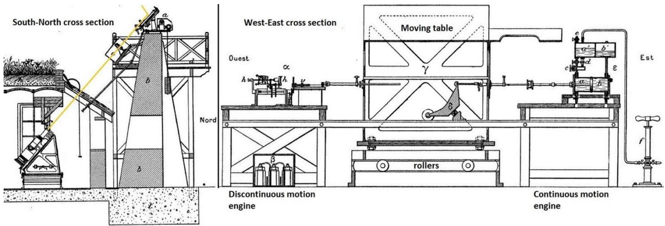
Figure 13. Side and face views of the spectroheliographs installed by Deslandres in the “ Petit Sidérost at” laboratory (1898). Left (side view): the polar siderostat (a), the imaging objective (c) and the spectroheliographs. Right (face view): the spectroheliographs are fixed upon an inclined table ( \gamma ), moving on rollers, and containing the polar axis. The first engine (East) is for the continuous translation needed for Call K spectroheliograms (the “ spectrohéliographe des formes ”), which moved under the action of the hydraulic motor ( \epsilon ) and the piston between water reservoirs (a, b). The second mechanism (West) is for the step motion required for the section spectroheliograph (the “ spectrohéliographe des vitesses ”) dedicated to radial velocities, using the electric motor ( \alpha ), the step engine (h) of Figure 15 and the set of batteries \beta . After Deslandres, 1905 b .
