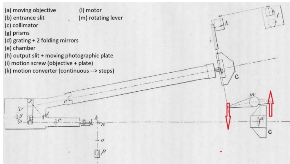
Figure 17. The new section spectroheliograph at the “Petit Sidérostas” in 1906, denoted (c) in Figure 16. It uses either three prisms for Call K (g) or a plane grating for H \alpha . (l) is a motor acting simultaneously on the entrance objective (a) and the photographic plate (h) through the (k) mechanism, which converts the continuous rotation of the motor (l) into step motions (details in Figure 15). (i) is a rotating screw translating the plate; (m) is a fixed pivot point with two levers of different lengths, in order to adapt the ratio of the translation velocities of (h) and (a) to the optical magnification of the spectrograph (as in Figure 6). After Deslandres (1910).
