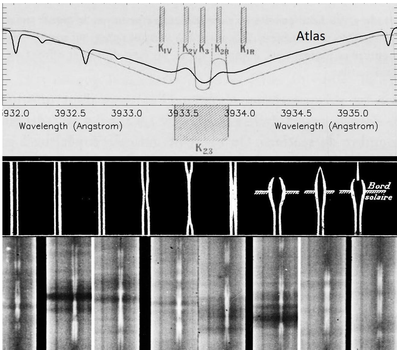
K2v, K2r drawings and K line observations at various locations
