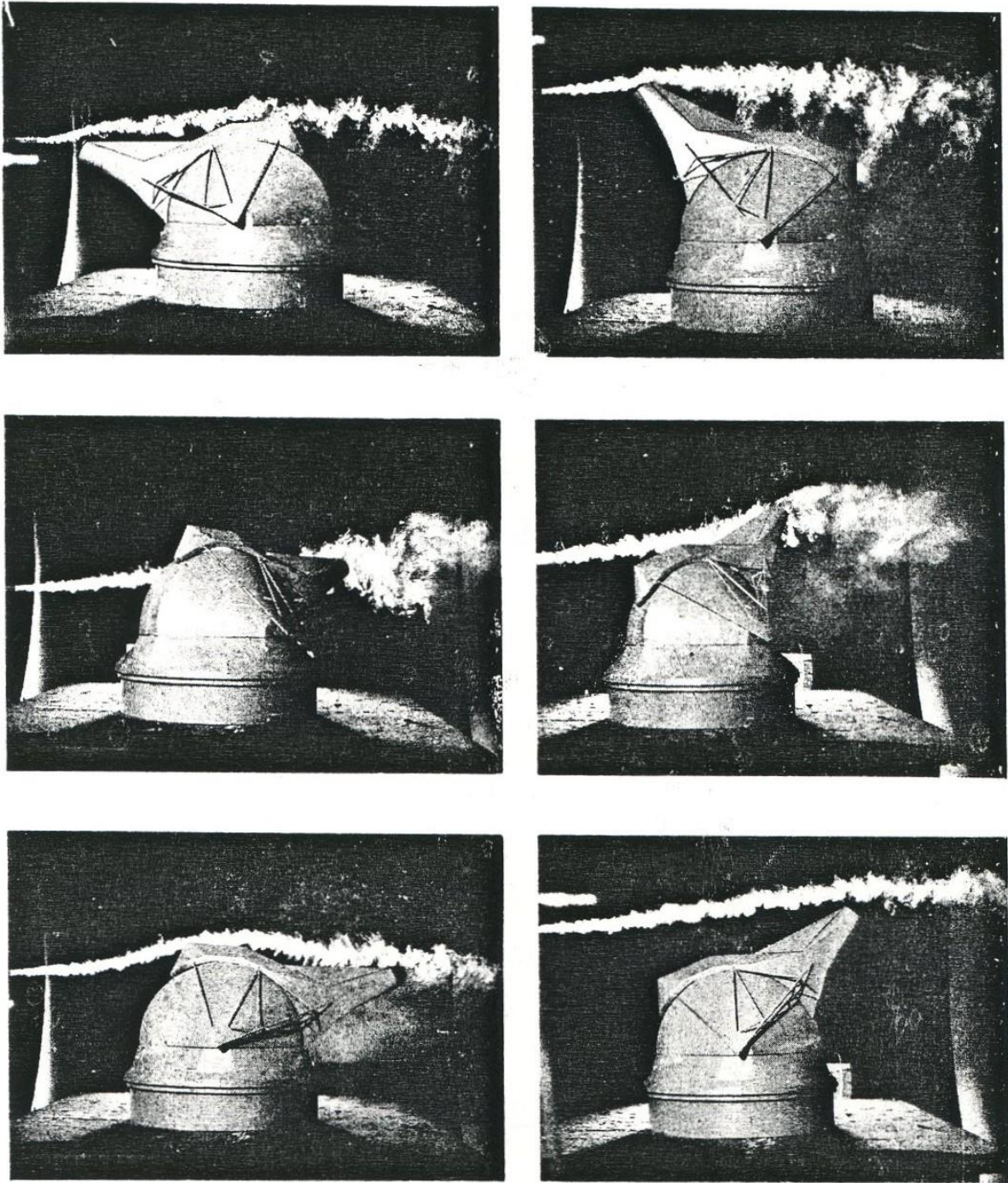
Figure 2: A reduced model of the dome and helmet was tested in a wind tunnel to study the occurrence of turbulent flows under various conditions (courtesy OMP).
