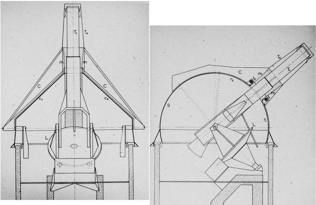
Figure 3: Drawings of the Turret-Dome (1960). C, c 1 , c 2 , T 2 = helmet structure; g = dome; T 1 = refractor tube; j, m = flexible washers; r 1 , r 2 = rolling curtains; L = equatorial table and fork (courtesy OMP).
