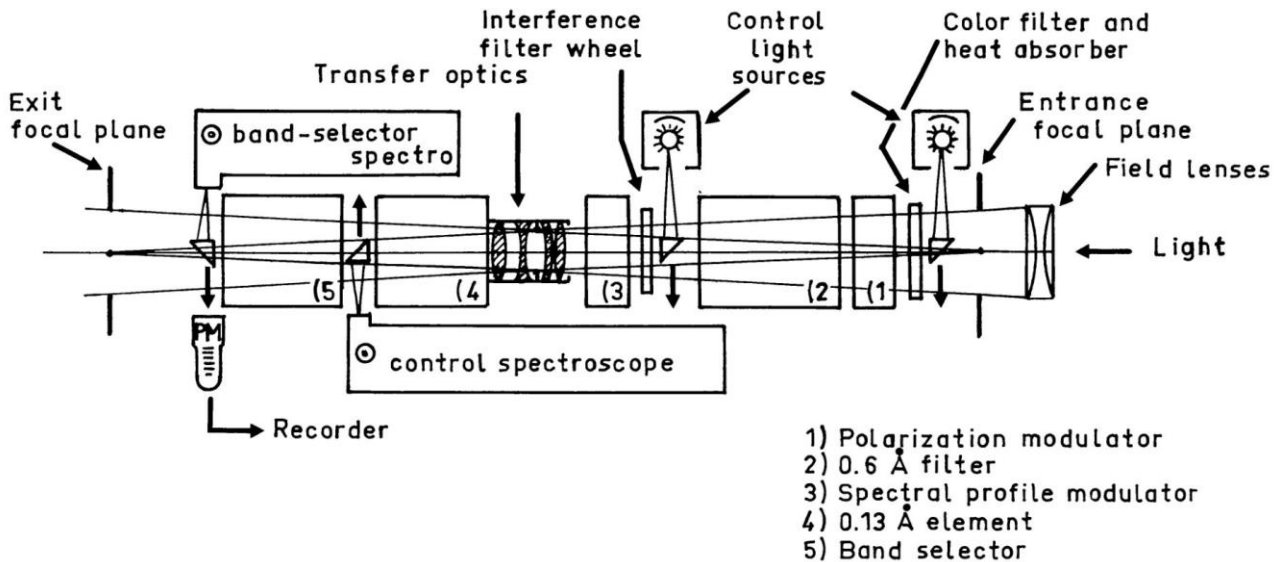
Figure 8: The "Filtre Polarisant Solaire Selectif" (FPSS) developed at Meudon and installed on the Turret-Dome in 1992 was composed of two Lyot filters and a polarization modulator. After Dollfus et al. , 1985.
