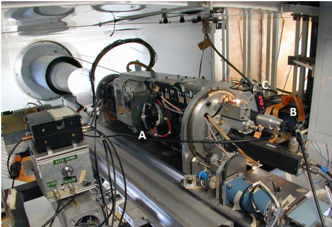
Figure 22: The heliometer mounted in the Turret-Dome. A: servomotor for scanning the light beam (producing the solar limb profiles). B: the output signal recorded through a photomultiplier. C: the digital image slicing counter, a key piece to be sure to pass through the true solar diameter after measuring several chords above and below. The whole system (about 40 kg) was rotating around the optical axis. Courtesy OCA.
