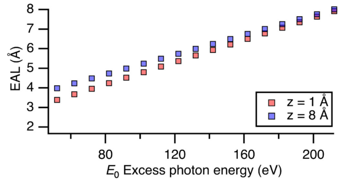
FIG. 4. EAL as a function of photoelectron kinetic energy calculated for P3HT at z = 1 Å (orange squares) and z = 8 Å (purple squares).
