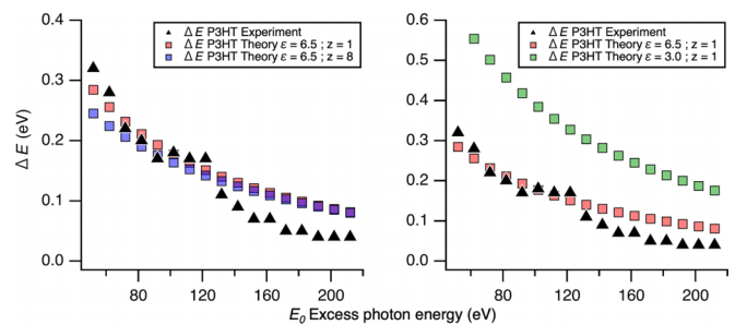
FIG. 5. Left: Calculated PCI shift for P3HT at z = 1 \text{ \AA} (orange squares), z = 8 \text{ \AA} (purple squares). Right: Calculated PCI shift for P3HT at \epsilon = 3 (green squares), \epsilon = 6.5 (orange squares). Experimental data in black triangles.
