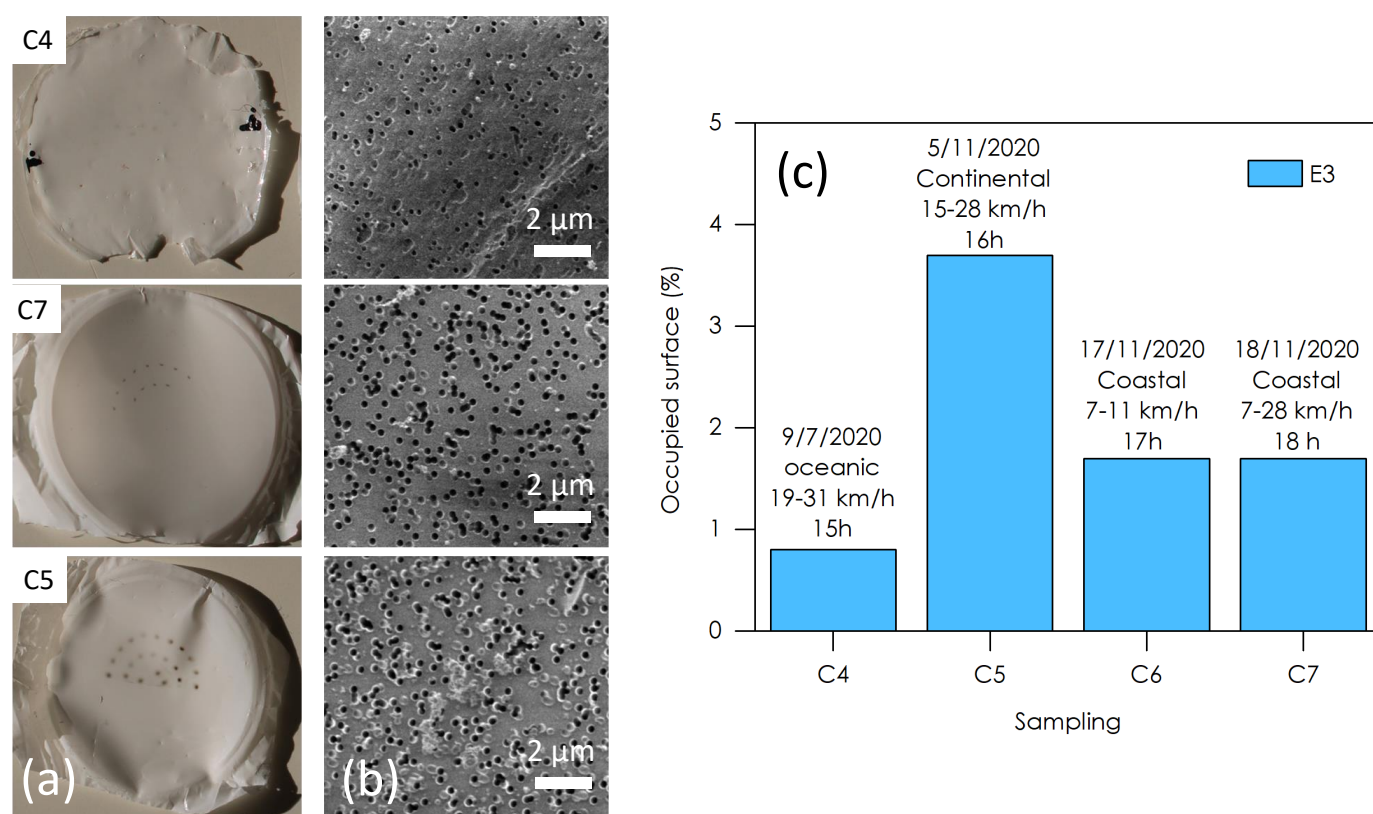
Figure 8. (a) Photograph of the polycarbonate filters of the E3 stages of three samples taken at Le Croisic under different air mass conditions: oceanic (C4), continental (C5), and coastal (C7). (b) Typical SEM images used for particle density measurements. (c) Particle density per unit area for 4 samples from Le Croisic (C4, C5, C6, and C7).
