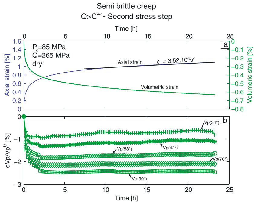
Figure 9. (a) Evolution of the axial and volumetric strains during the second creep step for the experiment done at P_c = 85 MPa. (b) Evolution of the \delta V_p/V_p^0 with respect to \sigma_1 during this creep step.
