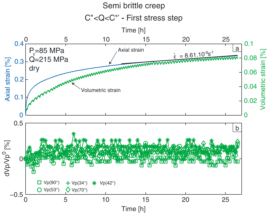
Figure 8. (a) Evolution of the axial and volumetric strains during the first creep step of the experiment done at P_c = 85 \text{ MPa} . (b) Evolution of the \delta V_p/V_p^0 at different angles with respect to \sigma_1 during this creep step.
