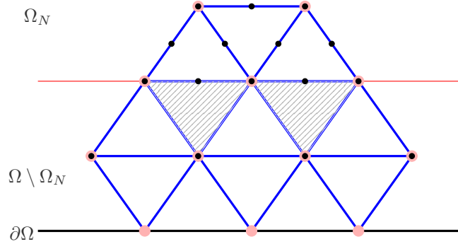
Fig. 3: Finite element pair which does not fulfill the inf-sup condition. The degrees of freedom for the components of the velocity are in black, those for the pressure are in pink. The two hatched elements include 4 degrees of freedom for each of the components of the velocity.
