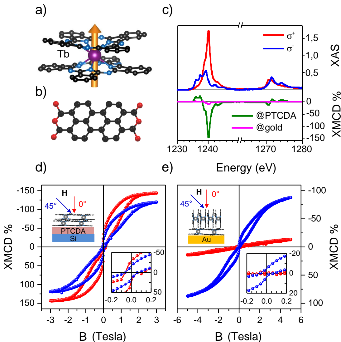
Figure 1 a) TbPc 2 molecule; carbon atoms are shown in black, nitrogen in blue, terbium in purple, hydrogen atoms are not shown. The orange arrow represents the J=6 total angular
