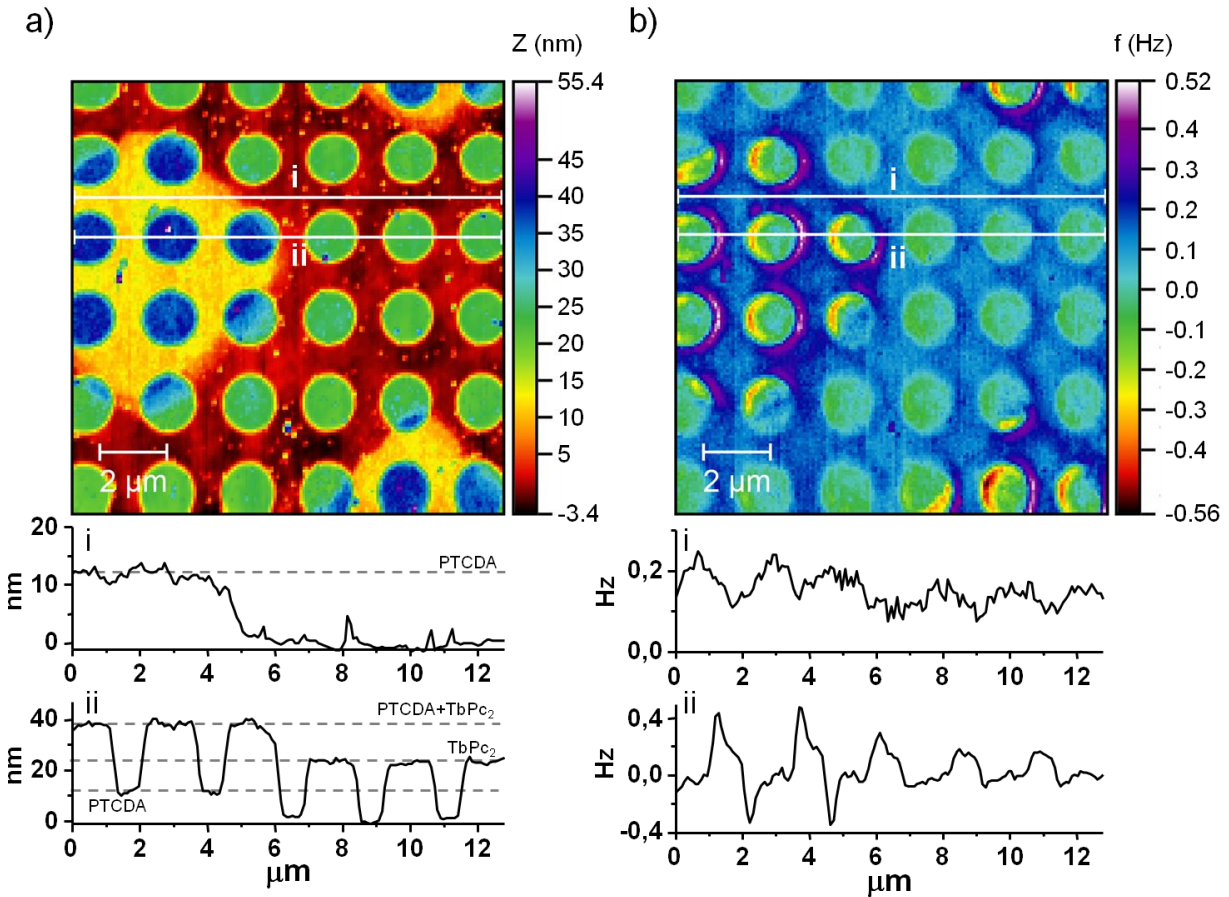
Figure 2 a) Topography of the \text{TbPc}_2 dot microarray on patterned PTCDA layer on silicon, measured at 10 K. The profiles along the lines i and ii are shown at the bottom, indicating that \text{TbPc}_2 structures are 24 nm thick, while PTCDA squares are 12 nm thick; the approximate heights of the structures are indicated with dashed lines. b) MFM image at a lift height of 85 nm from the surface, measured together with a) at 10 K and 4 Tesla. The MFM frequency shift profiles along the same i and ii lines measured in the topography are shown at the bottom.
