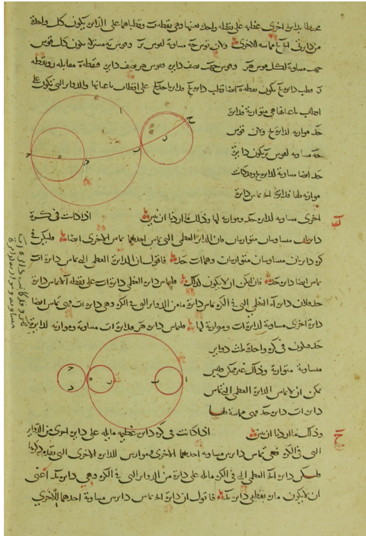
FIGURE 1. From Theodosius' Spherics . On the top, the figure for Proposition II.6. Ms. 3464, fol. 30, Topkapi Saray, Ahmet III.
