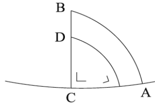
FIGURE 7. Proposition 41 fails when AB and AC are greater than a quarter of a circle
