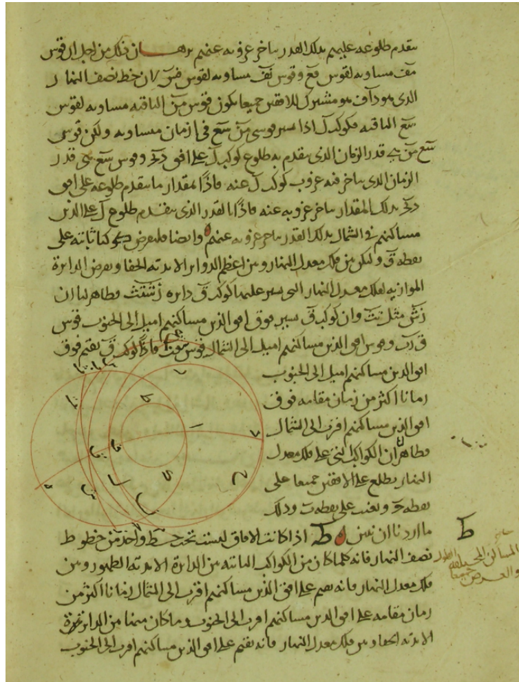
FIGURE 19. From Theodosius' Habitations ; at the bottom of the page, the statement of Proposition 9 and the corresponding figure. Version of Qusṭā ibn Lūqā, Ms. 3464, fol. 121, Topkapi Saray, Ahmet III.
