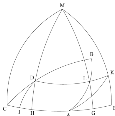
FIGURE 5. Figure for Proposition 41
