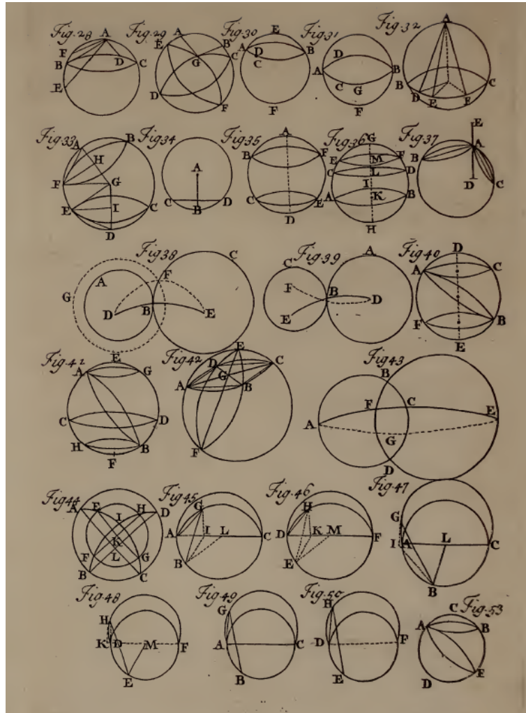
FIGURE 2. A plate of figures for Book II of Theodosius' Spherics , Clavius' edition [8].
