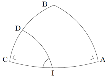
FIGURE 6. Proposition 41 fails with the assumption that AB and BC are equal to a quarter of a circle
