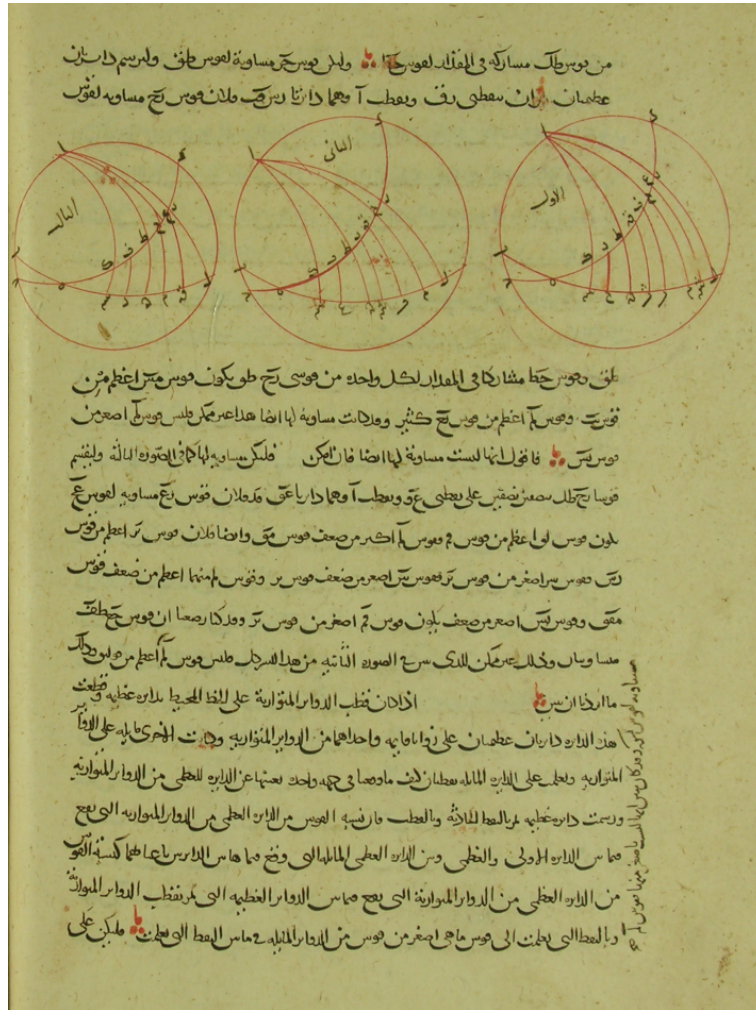
FIGURE 4. From Theodosius' Spherics , Proposition III.10. Ms. 3464, fol. 50, Topkapi Saray, Ahmet III.
