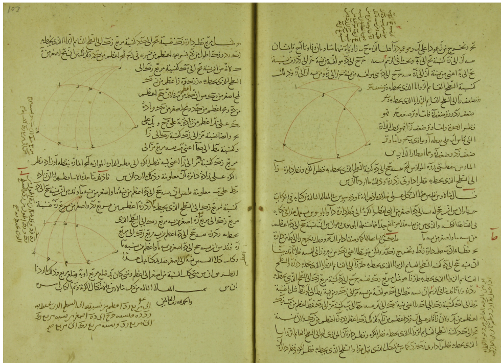
FIGURE 15. Propositions 89 to 91 of the Spherics , Ms. 3464, fol. 99, Topkapi Saray, Ahmet III.
