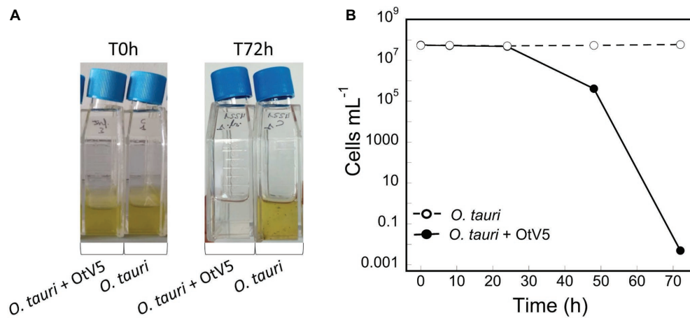
FIGURE 2 | Dynamics of the infection of O. tauri with OtV5. (A) Infection and control culture flasks at time 0 and 72 h. (B) O. tauri cell abundances (average ± standard error) detected by catalyzed reporter deposition fluorescence in situ hybridization and counted by epifluorescence microscopy in both the infected (solid circles) and the control (empty circles) triplicate cultures.
