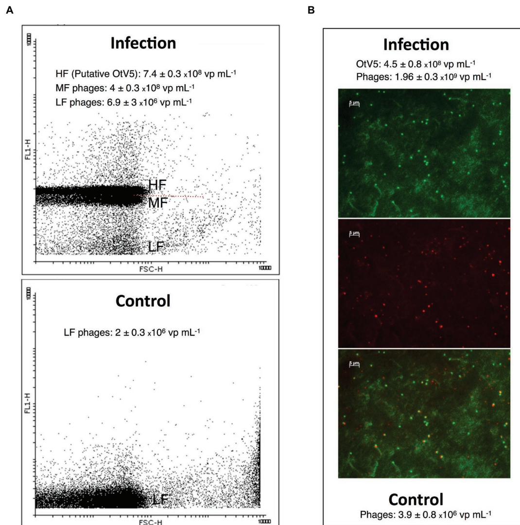
FIGURE 5 | Comparison of free virus counts using flow cytometry (FCM) and virus fluorescence in situ hybridization (VirusFISH). (A) Cytogram of viral events from an infected (96 h after OtV5 inoculation, upper panel) and a healthy O. tauri culture (Control, lower panel). The cytogram of the infected culture shows mid-level (MF) and high-level (HF) fluorescence viruses (presumably phages and putative OtV5), and also low-level fluorescence viruses (LF). The dashed red line separates MF from HF virus. Only LF viruses (phages) are seen in the control. (B) Micrographs of the 0.02 \mu\text{m} filter of an infected culture. Top: total viruses stained with SYBR Gold. Center: VirusFISH labeled OtV5 viruses. Bottom: overlay of SYBR Gold and VirusFISH signals for OtV5 viruses. Values in the graphs represent the values obtained with VirusFISH (on the 0.02 \mu\text{m} filter) and flow cytometry for the same 0.2 \mu\text{m} prefiltered samples for both the infected and the healthy O. tauri culture.
