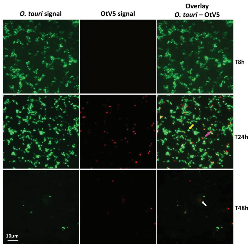
FIGURE 3 | Micrographs of the evolution of the infection from time 8 to 48 h. Left: O. tauri only. Centre: OtV5 only. Right column: overlay of O. tauri host cells in green (Alexa488) and virus in red (Alexa594). Yellow arrow: non-infected O. tauri , pink arrow: infected O. tauri , gray arrow: cloud of viruses retained on the filter by the organic matter released during the lysis. See supplementary Figures for a complete temporal overview of both the infection and the control cultures.
