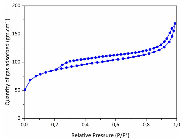
Fig. 3 N 2 sorption isotherms of the PSZNi2.5_5 sample.
