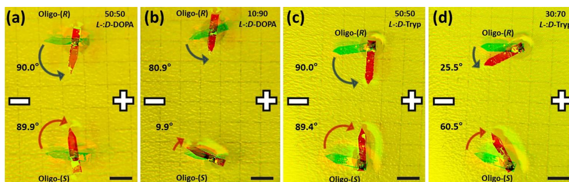
Figure 3. Optical pictures of the dynamic response of two monofunctional rotors, oligo-(R) and oligo-(S), obtained during the respective bipolar electrooxidation of enantiomeric mixtures; L-:D-DOPA ratios (a) 50:50 and (b) 10:90, and L-:D-Tryp ratios (c) 50:50 and (d) 30:70, in a 5 mM LiClO 4 solution.
