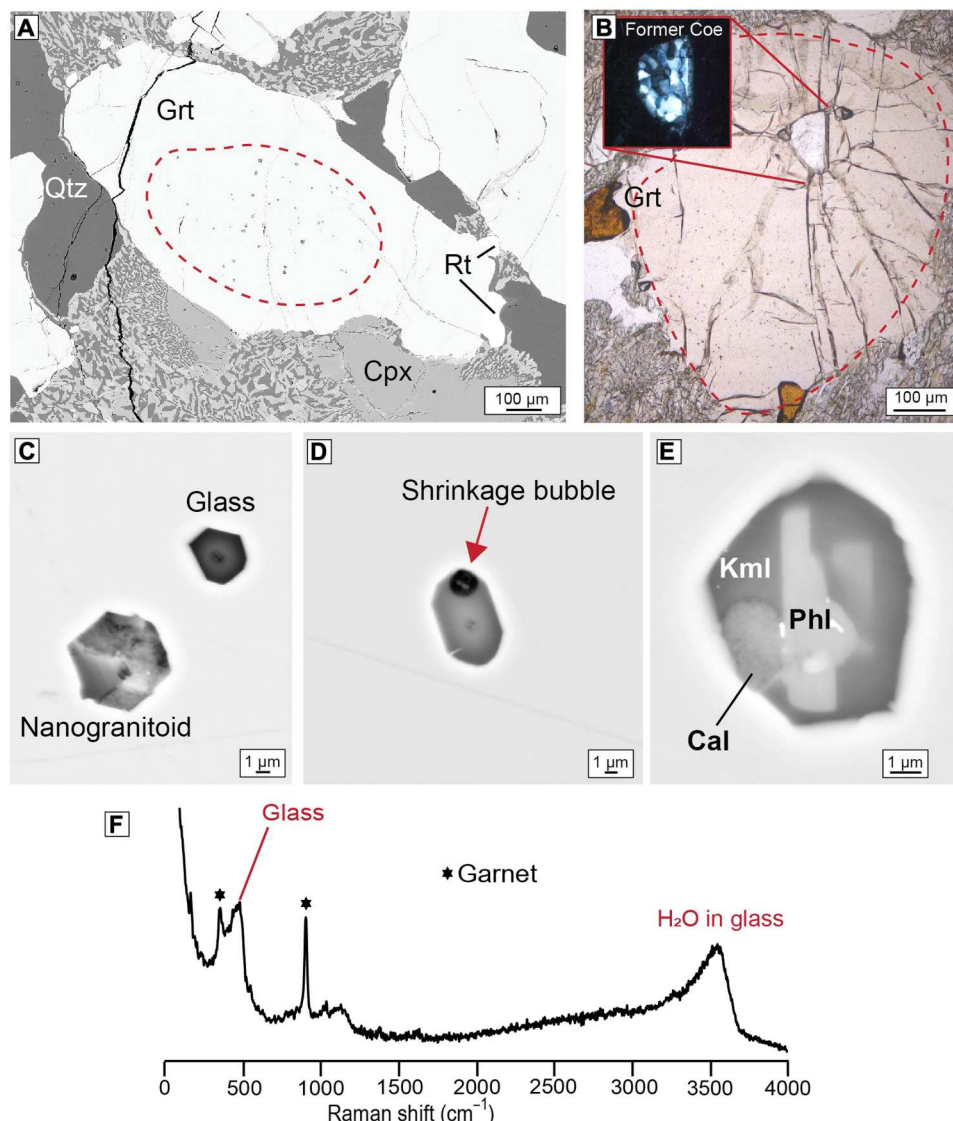
Fig. 1. UHP eclogites of Saidenbach, Erzgebirge, Germany. Backscattered electron (BSE) image (A) and photomicrograph (B) of eclogite texture and BSE images of melt inclusions (C to E). (A) Eclogite dominated by garnet (Grt) and clinopyroxene (Cpx) with minor quartz (Qtz) and accessory coarse-grained rutile (Rt). Grt contains a cluster of melt inclusions (dashed red line). (B) Detail of Grt with inclusion of polycrystalline quartz (in the red box inclusions in cross-polars) surrounded by radial cracks and interpreted as former coesite (Coe), in the same microstructural position with the cluster of melt inclusions (dashed red line). Melt inclusions are randomly distributed; they are both glassy (C and D) and crystallized as nanogranitoids (C to E). Some glassy inclusions contain a shrinkage bubble (red arrow) (D). The darker spots visible in the middle of the glassy inclusions are beam damages due to analysis. (E) Nanogranitoids are bigger than glassy inclusions; they have a regular shape that mimics that of the host mineral (i.e., negative crystal), and they consist of kumdykolite (Kml), phlogopite (Phl), calcite (Cal), kokchetavite, and quartz. (F) Raman spectrum of a preserved glassy inclusion in which the OH bands are visible.
