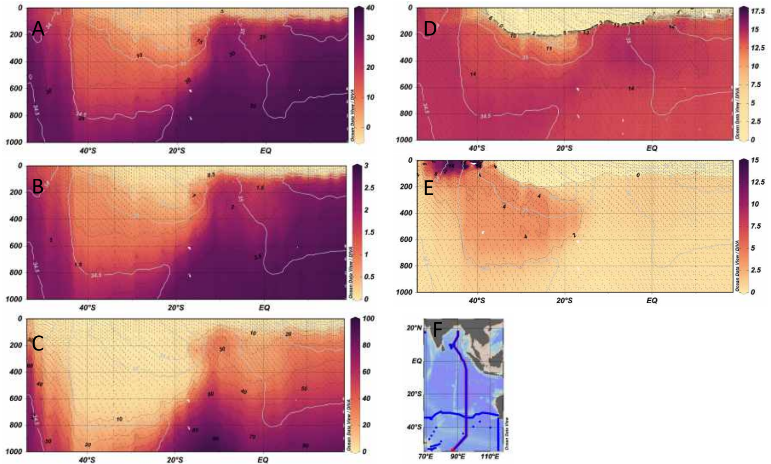
Figure 11: Vertical sections nominally along 90°E of A) nitrate ( \text{mmol m}^{-3} ) B) phosphate ( \text{mmol m}^{-3} ), C) silicate ( \text{mmol m}^{-3} ) D) nitrate to phosphate ratio, E) nitrate to silicate ratio, F) map of the section. The grey contours are salinity, and the black contours the colored property. The station locations for each property are shown as dots. Data from the World Ocean Database (2018), comprising mainly data from the IO9N and IO8S repeat hydrography lines. Only data from the 90°E N-S section are used in the section plots.
