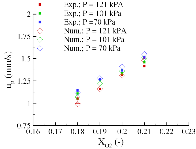
Figure 5. Spread rate as a function of X_{O_2} for different pressures. The oxidizer velocity is 150 mm/s and the Type#2 wire is considered.
