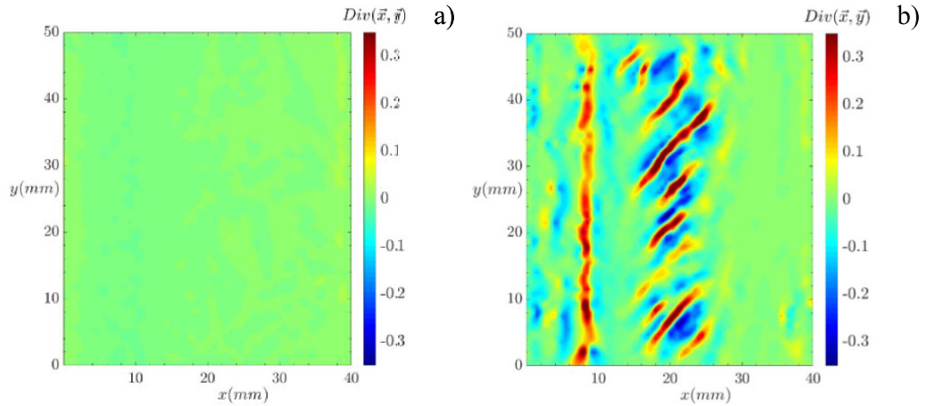
Figure 9. Patterns of the divergence of the displacement vector (\vec{\nabla} \cdot \vec{d}) corresponding to \Delta T \approx 7 K in the microgravity phase: (a) V_0 = 0 , (b) V_0 = 1.41 kV.
