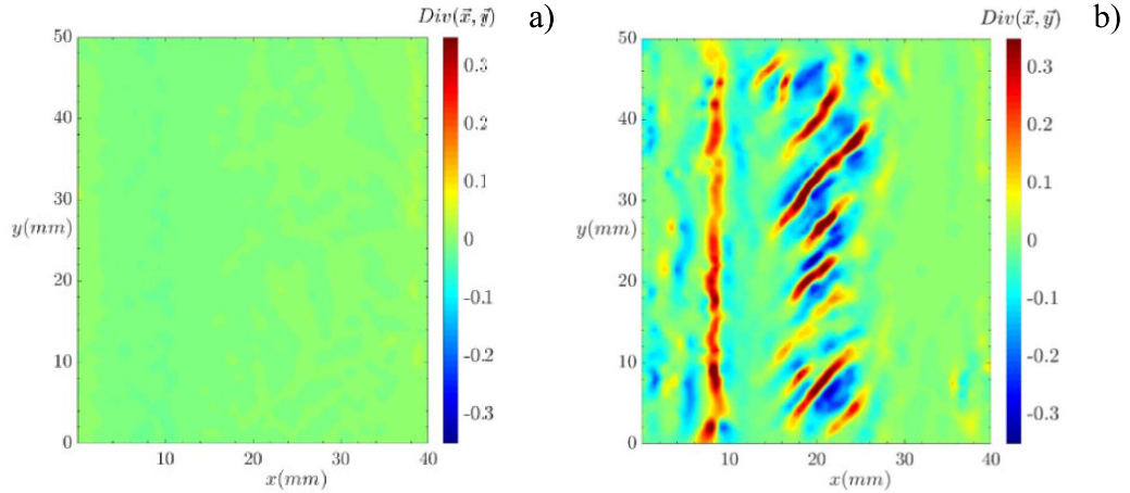
Figure 9. Patterns of the divergence of the displacement vector (\vec{V} \cdot \vec{d}) corresponding to \Delta T \approx 7 K in the microgravity phase: (a) V_0 = 0 , (b) V_0 = 1.41 kV.
