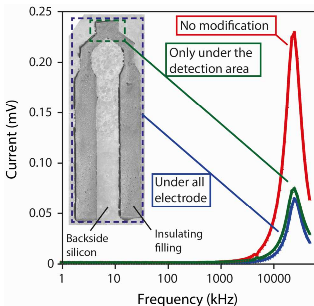
Figure 4: Three different backside designs (Red: Si-only, green: detection area-limited modification, and blue: extended to the electrode area modification) were fabricated and frequency responses of the devices were measured. The y-axis corresponds to the current value after the trans-impedance amplifier. Modified versions performed better at high frequencies by decreasing parasitics. Inset: The SEM image of the modified backside with PDMS filling. The green rectangle corresponds to the detection-area limited modification version.
