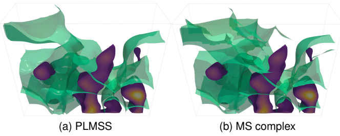
Fig. 8. Comparison of the PLMSS region boundaries and the MS complex using the Viscous Fingering dataset [67] simplified with an absolute persistence threshold of 0.1. Both images show the boundary interface of viscous fingers as contours of the salt concentration density scalar field, colored by the density from yellow (high concentration) to purple (low concentration). (a) shows that the PLMSS region boundaries can extract the region-separating geometries that separate single viscous fingers effectively without cluttering the visualization. (b) provides the original MS complex, where more geometry is extracted due to the saddle-saddle 2-cells, cluttering the image. Those saddle-saddle walls would have to be removed by additional postprocessing.
