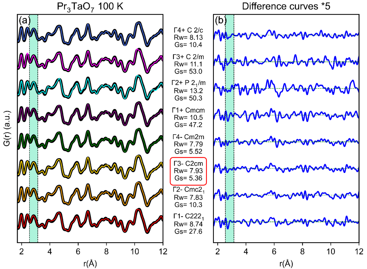
Figure 6: (a) Neutron pair distribution function (PDF) of weberite-type Pr 3 TaO 7 measured at 100 K (black circles) and refined with the long-range Cmcm space group (purple) and with the models derived at the Brillouin zone center (red, orange, gold, green, cyan, magenta, and royal blue) of Cmcm . The four non-centrosymmetric models ( \Gamma_{1-4}^- ) are the bottom curves and the four centrosymmetric models ( \Gamma_{1-4}^+ ) are the top curves. (b) Difference curves (multiplied by a factor 5) between as-collected data and respective models in the r -range between 1.7 – 12 Å. The turquoise shaded area enclosed by the vertical dashed lines between 2.5 and 3 Å highlights the region most sensitive to the O-O atomic correlations. The red box around the C2cm space group highlights the best structural model to describe the PDF of Pr 3 TaO 7 .
