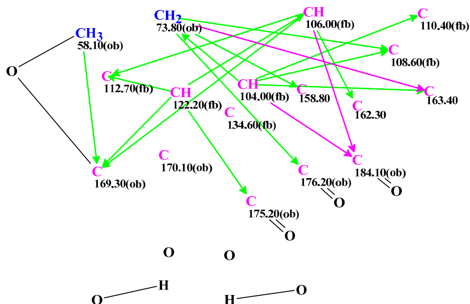
Figure 4. Molecular Connectivity Diagram obtained from the NMR data of ominoxanthone ( \text{C}_{17}\text{H}_{10}\text{O}_8 ) recorded in TFA- d . Carbons hybridized as sp^3 and sp^2 are respectively written in navy blue and violet. The admissibility of a neighbor heteroatom is indicated by the labels « ob » (obligatory) and « fb » (forbidden). HMBC connectivities are indicated by green arrows. Violet arrows refer to nonstandard correlations (length n > 3 , for ^nJ_{\text{HH,CH}} ). These correlations were set for the weak HMBC signals.
