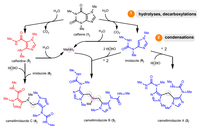
Figure 1. The (bio)chemical logic of camellimidazoles formation.
