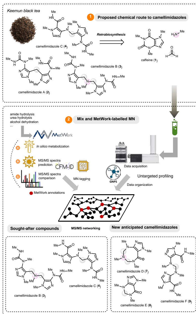
Figure 2. Overview of the analytical workflow developed in this study along with the structures of the obtained compounds.
