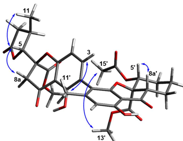
Fig. 4. Key ROE correlations of compound 2.
