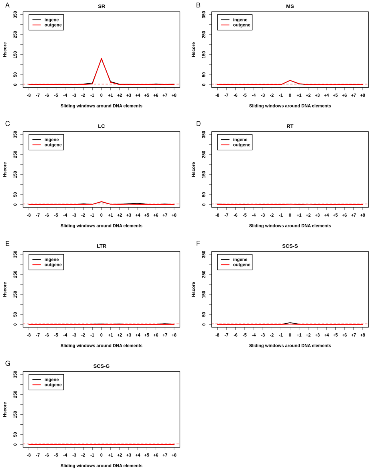
Figure 4. DNA repeats hotspotness relative to genes is dependent upon their type. High-copy DNA repeats: (A–C). (A) Simple Repeats (SR). (B) MiscoSatellites (MS). (C) Low Copy repeats (LCR). Viral origin DNA repeats: (D) Retro-Transposons (RT). (E) Long Terminal Repeats (LTR). Low copy repeats: Selfchains segments (SCS) (F,G). (F) Selfchains segments of type self aligned (SCS-S). (G) Selfchains segments of type Gapped (SCS-G). Horizontal red dashed line corresponds to Hscore threshold of 3 for hotspotness.
