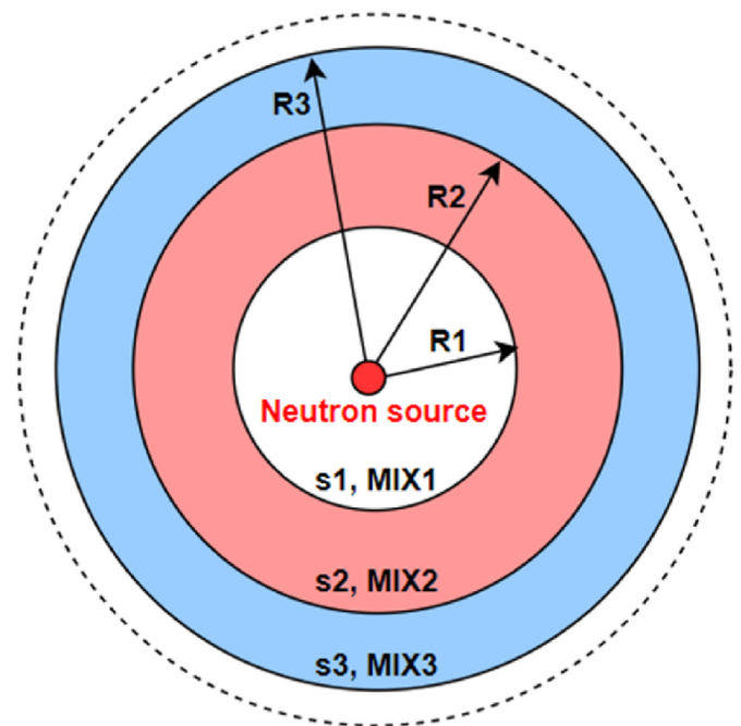
Fig. 1. Geometry context used for generating the spectra dataset with Serpent; s_{1,2,3} represent the surfaces; R_{1,2,3} represent the radii; MIX _{1,2,3} represent the material mixtures; dashed sphere represents the detector.
