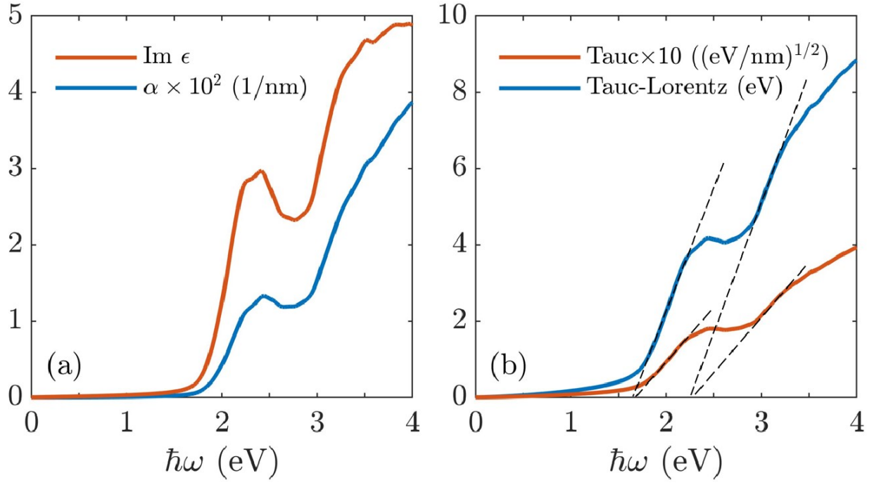
FIG. 5. (a) Imaginary part of the dielectric function and absorption coefficient of \text{U}_3\text{O}_8 . (b) Tauc and Tauc-Lorentz plots, often used in experiment to determine indirect band gap values. As explained in the main text, in the present case the linear extrapolations to the abscissa (represented by the dashed lines) lead to values not directly related to the band gap in \text{U}_3\text{O}_8 .
