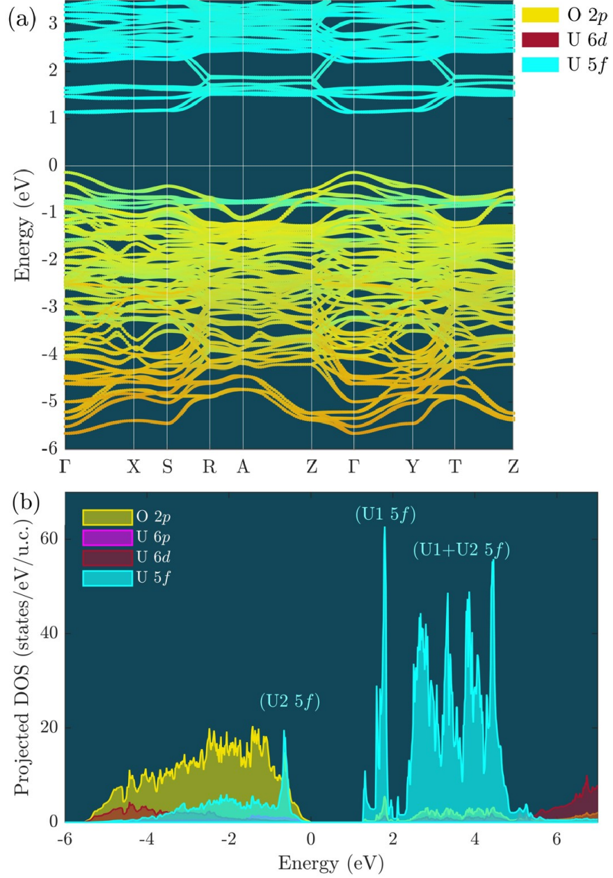
FIG. S2. (a) Band structure of \text{U}_3\text{O}_8 , with the colors highlighting the contributions of the U 5f, O 2p, and U 6d states, which are the main contributors in the energy range shown [the valence band maximum (VBM) is at 0]. The \mathbf{k} -point path used is shown in Fig. S3. (b) Atom-type projected density of states. The density of states calculations indicate that the band gap is close to 1.27 eV. The U1 and U2 5f labels are for reference in the main text.
