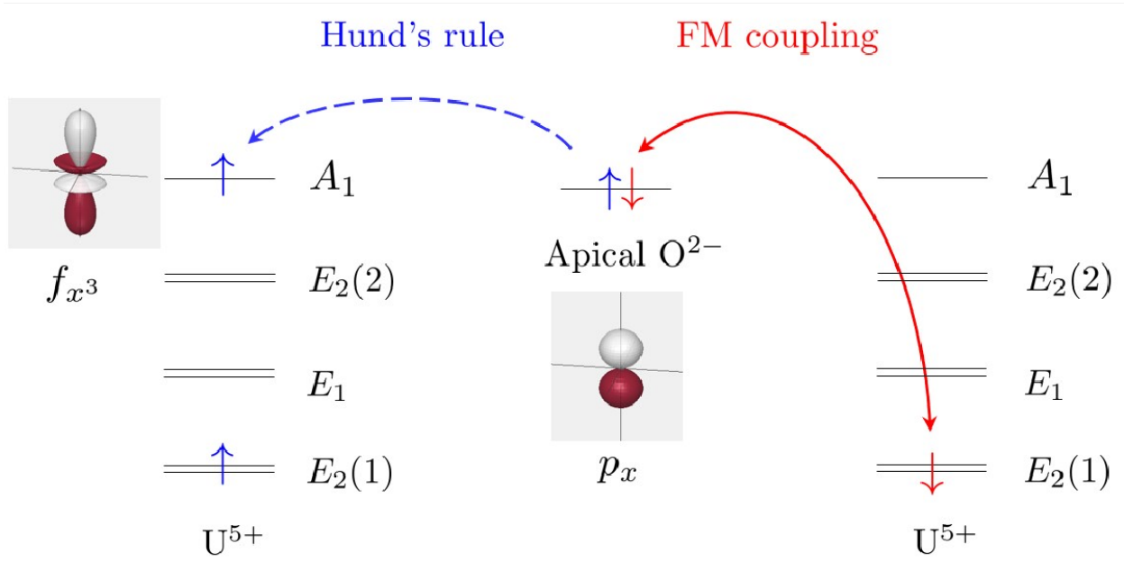
FIG. 4. Illustration of the Anderson-Goodenough-Kanamori rule for AFM superexchange coupling in the 180^\circ U 2 -O-U 2 configuration. Thanks to orbital overlap, an oxygen ion electron is virtually excited to a neighboring U 2 ion, with a spin complying to Hund's maximum spin rule. The unpaired electron on the O - ion, which has opposite spin, couples ferromagnetically to the other U 2 ion. This is because the p_x orbital is orthogonal to the E_2(1) states. The effective U 2 -U 2 coupling is AFM.
