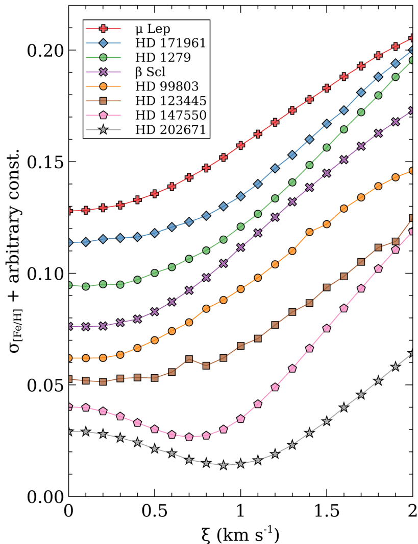
Figure 8. Microturbulent velocity determinations for the eight stars
