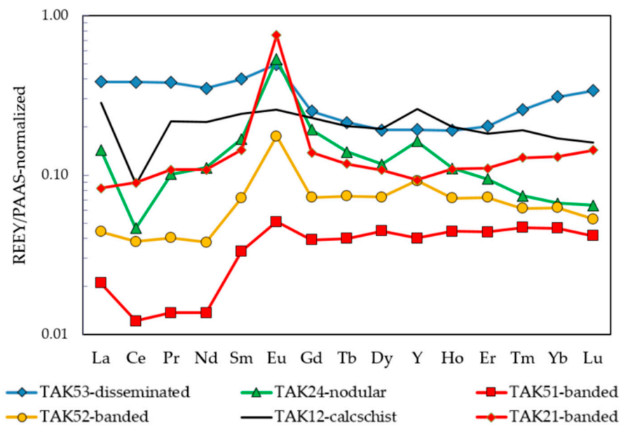
Figure 5. REE and Y patterns of the ore samples and calcschist (TAK12) from Takab. Normalization values to Post-Archean Australian Shale (PAAS) from [31].
