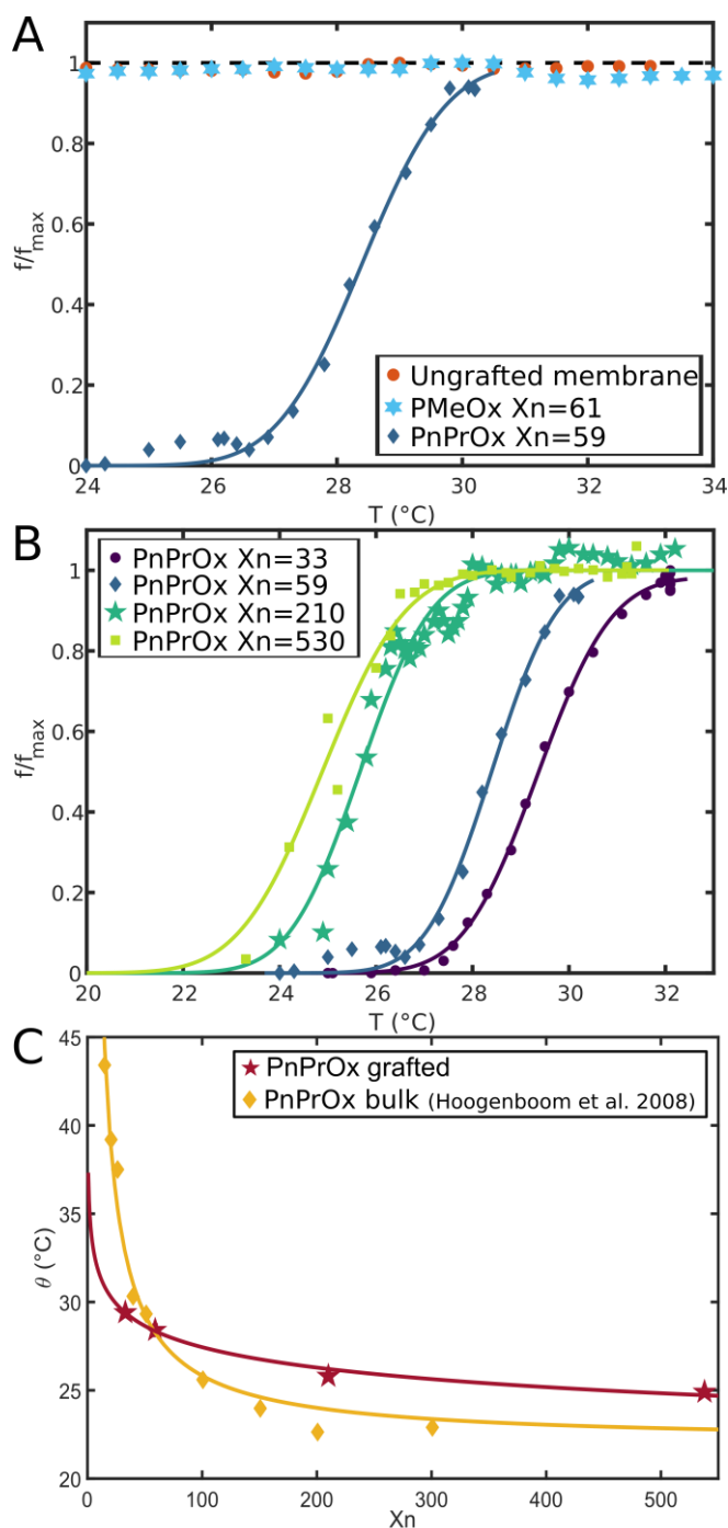
Figure 2: Normalized translocation frequency as a function of temperature for differently grafted pores. A) Comparison of the frequency of translocation of \lambda -DNA as a function of temperature for PMeOx ( X_n=61 ), PnPrOx ( X_n=59 ), and ungrafted membrane. Pore diameter 42 \pm 0.5 nm. Applied pressure: 80 mbar. The blue solid line represents the fitting by the error function. The dashed black line represents the constant f/f_{\max}=1 . Unaveraged curves are shown in Supplementary Information S8 . B) Comparison of the frequency of translocation of \lambda -DNA as a function of temperature for different number-average degree of polymerization of PnPrOx ( X_n=33 , X_n=59 , X_n=210 , X_n=538 ). Pore diameter 42 \pm 0.5 nm. Applied pressure: 80 mbar. Solid lines represent the fitting by error function. Unaveraged curves are shown in Supplementary Information S8 . C) Transition temperature \theta for different polymerization degrees X_n . Red stars correspond to the PnPrOx graftings used in this study. Yellow diamonds correspond to a study from Hoogenboom et al. (22). Solid lines represent model fitting with a power
