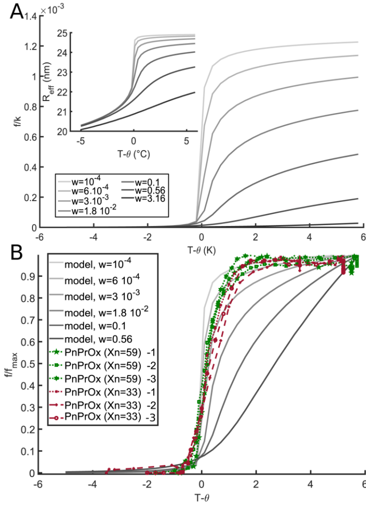
Figure 3: Theoretical modeling of the gating phenomenon. A) (main) Modeling of the frequency of translocation normalized by the suction model prefactor k . This prefactor corresponds to the frequency of translocation for P=P_c . (inset) Modeling of the effective radius of the grafted nanopore, R_{eff} , as a function of temperature difference T-\theta with \theta the critical temperature. Different values of the third virial coefficient w are represented by different colors. B) Comparison between the coarse-grained model and individual translocation experiments (numbers 1 to 3) for different PnPrOx graftings ( X_n=33 and X_n=59 ) normalized by the maximum frequency f_{max} .
