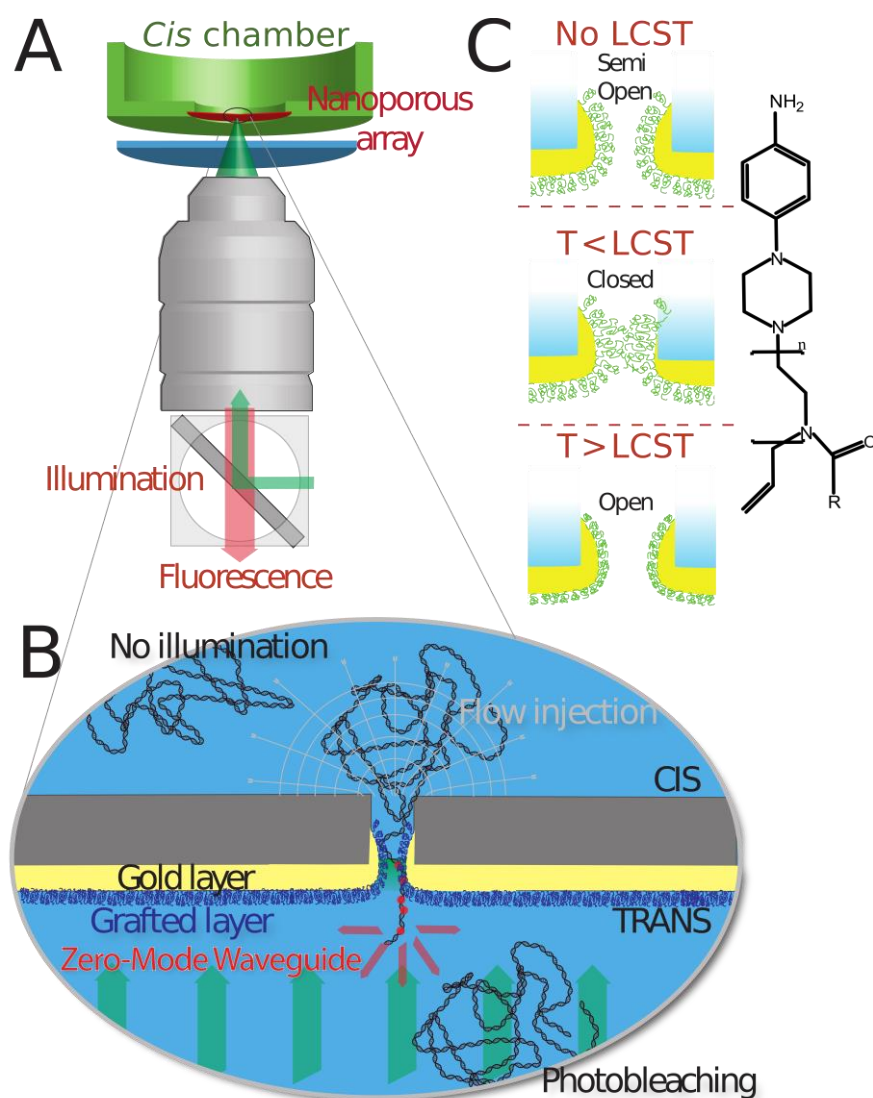
Figure 1: Zero mode waveguide setup for nanopore with grafted polymer. A, B) Schematic of the zero-mode waveguide (ZMW) for nanopores setup. It uses a nanoporous array coated with a gold layer for near-field enhancement. When illuminated with a laser, the fluorescent molecules in the cis chamber do not receive any light because of metal whereas downstream molecules are unfocused and bleached by the laser. Only the fluorescent molecules in the pore in the vicinity of the metal film are exposed to an enhancement of the electromagnetic field which leads to reinforcement of the fluorescence. This methodology enables the detection of single molecules translocation events with a high parallelization. In the case of nanoporous arrays functionalized with grafted polymers, the translocation of the transported molecule can be modulated by closing and opening the grafted channels. An exemplary video recording of the translocation events can be found in Supplementary Information S12 . C) Left: Schematic of how grafted polymers modulate the pore diameter. Polymers that do not exhibit a lower critical solution temperature ( LCST ) limit the channel size but cannot completely close the pore. Pores grafted with polymers with an LCST can be triggered by changing the temperature to switch from an open state at high temperature to a closed state at low temperature. Right: Poly(2-alkyl-2-oxazoline)s structure. The -R group corresponds to -CH 3 for PMeOx and for -CH 2 -CH 2 -CH 3 for PnPrOx.
