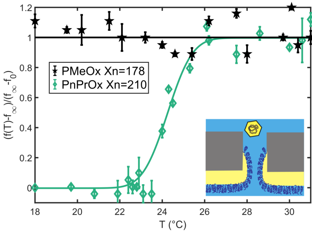
Figure 5: Controlled translocation of viral particles. Normalized frequency of translocation of AAV viral particles as a function of the temperature for two different graftings: black stars are PMeOx and green diamonds are PnPrOx. Pore diameter ( 220 \pm 1.8 ) nm. Applied pressure: 4 mbar. The green solid line is the result of fitting by an error function. Black solid line is the constant (f(T)-f_{\infty})/(f_{\infty}-f_0)=1 . N > 2 for each experiment. Errors bars are standard errors. Insert: Scheme of an AAV virus at the entry of a grafted nanopore.
