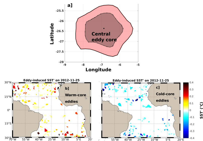
Figure 3. (a) A representative example of an eddy with its central-core, where the mean anomalies were computed. (b and c) Mean SST anomalies induced by warm-core and cold-core eddies on 2012/11/25. White areas are areas without eddies.
