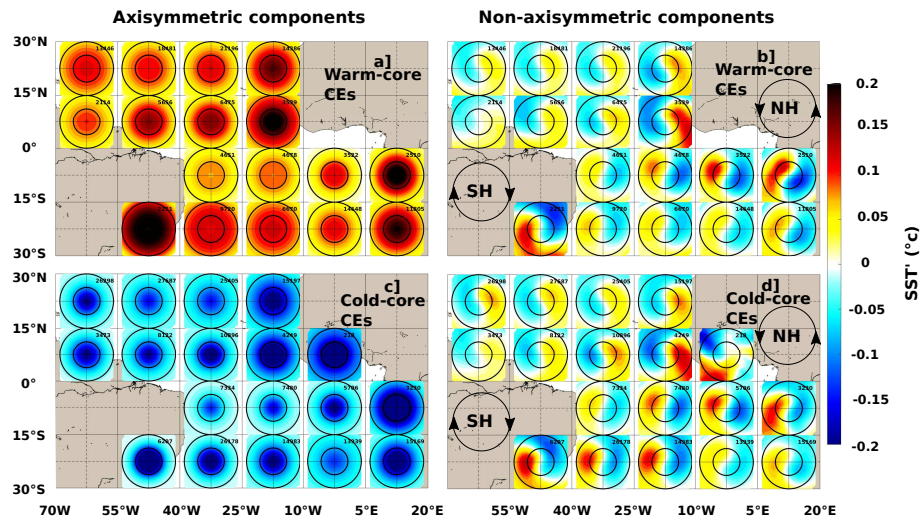
Figure 9. Same as Figure 7 for cyclonic eddies.
