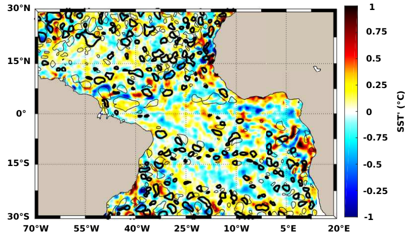
Figure 2. (a) High-pass filtered SST (background color) and detected eddies on 2012/11/25. Cyclonic and anticyclonic eddy edges are represented in thick and thin black contours, respectively.
