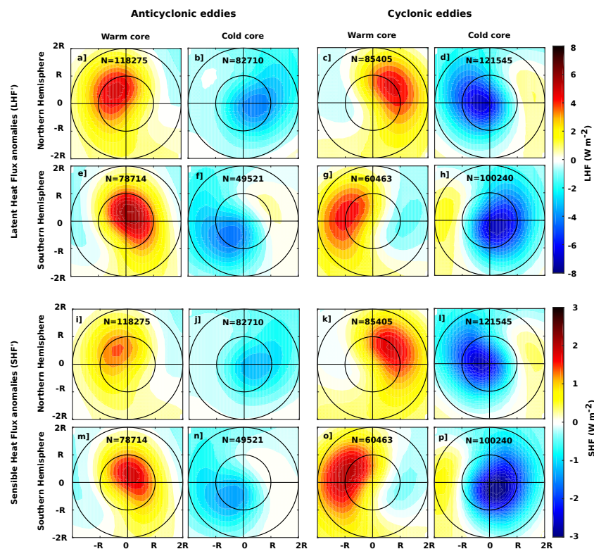
Figure 12. Same as Figure 5 for (a-h) latent and (i-p) sensible heat flux anomalies. The number average eddy composites is denoted N.
