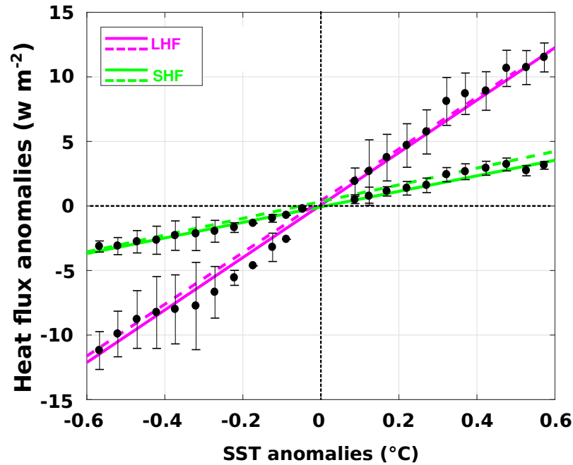
Figure 11. Eddy induced heat flux anomalies as function of SST anomalies (black dots) with the corresponding linear fitting for LHF (magenta full line) and SHF (green full line) anomalies. Dash lines indicate the linear fitting obtained when considering only the axisymmetric components of composites of SST and heat flux anomalies (see text). Error bars denote \pm 1 standard deviation.
