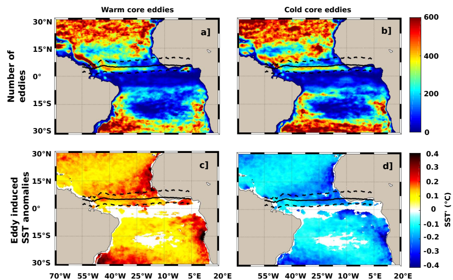
Figure 6. Distribution of (a–b) warm-core and cold-core eddies, and (c–d) eddy induced SST anomalies over the 2010 – 2017 period. Solid and dashed curves represent the mean annual and extreme (during boreal winter and summer) location of the ITCZ. White areas stand for areas where not enough eddies were available.
