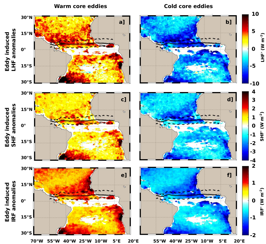
Figure 10. Distribution of latent heat flux (LHF) and sensible heat flux (SHF) and ocean infrared flux (IRF) anomalies over warm-core and cold-core eddies.
