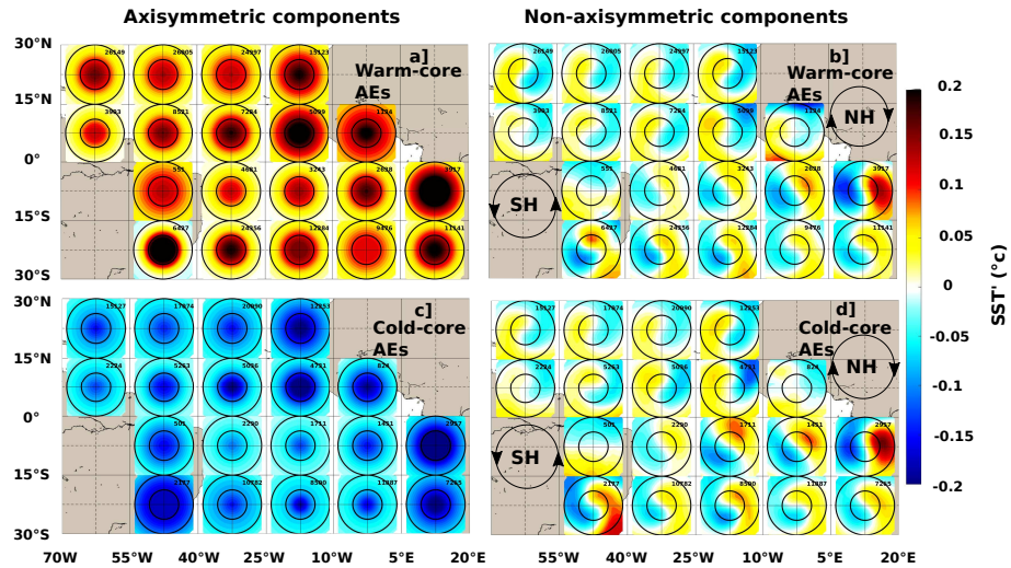
Figure 8. Distribution of (a,c) axisymmetric and (b,d) non-axisymmetric component of warm-core and cold-core anticyclonic eddies. Rotation direction of eddies are indicated in the Northern and Southern Hemisphere on black circles.
