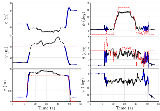
Figure 8. States performances of the drone in flight tests. Dotted red line is the desired reference for the vehicle. Blue line represents the states of the vehicle while being stopped. Hard blue line designs the states during flight mode Q_1 . Q_2 flight performances are represented in black solid line. Eventually, Q_3 mode is depicted in gray.
