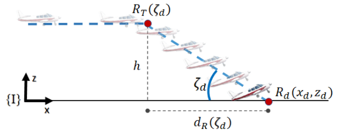
Fig. 1: Landing strategy in a specific coordinate for a fixed-wing drone with the least speed.
