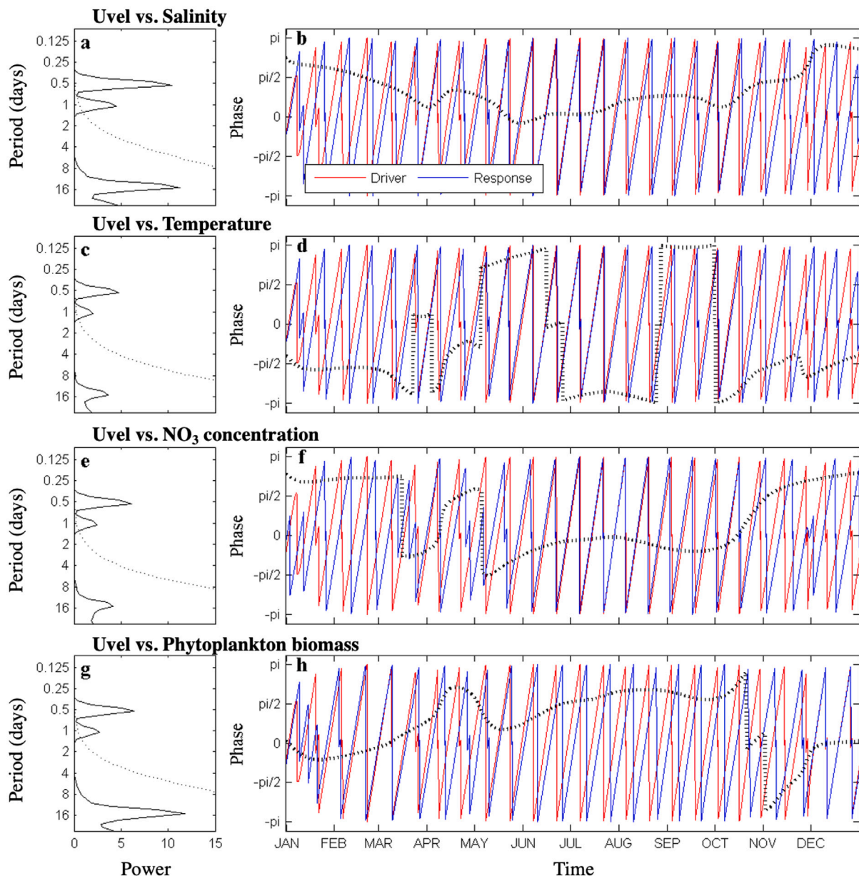
Fig. 10. Wavelet coherence analysis computed for the zonal component of current velocity (uvel; \text{m s}^{-1} ) versus (a, b) salinity, (c, d) temperature ( ^{\circ}\text{C} ), (e, f) nitrate concentration ( \text{NO}_3 , \text{mmol m}^{-3} ), and (g, h) total phytoplankton biomass ( \text{mmol N m}^{-3} ) for the 1-year simulation. Left-hand panels (a, c, e, g) show the average wavelet cross-spectrum. Dotted lines show the \alpha = 5\% significance levels computed based on 1000 Markov bootstrapped series. Right-hand panels show the phases of both time series computed for the peak of highest coherence: uvel (red line) versus (b) salinity, (d) temperature, (f) \text{NO}_3 , and (h) total phytoplankton biomass (blue lines). Dashed lines represent the phase difference between both signals.
