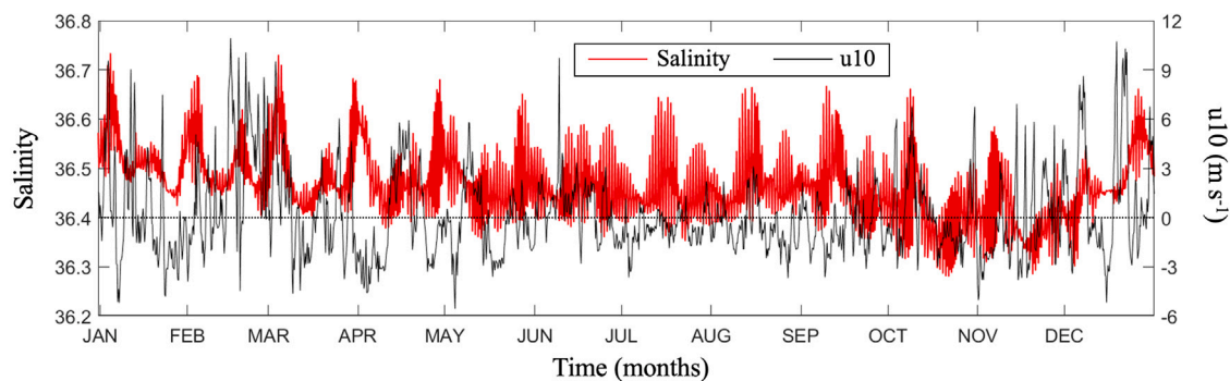
Fig. E.1. Temporal evolution of salinity versus the zonal component of the wind at 10 m ( u10 , \text{m s}^{-1} ) every 6 h at 6.11^\circ\text{W} and 36.06^\circ\text{N} (red circle in Fig. 1b). The black horizontal line represents the zero u10 reference delimiting positive (negative) values that indicate westerly (easterly) winds.
