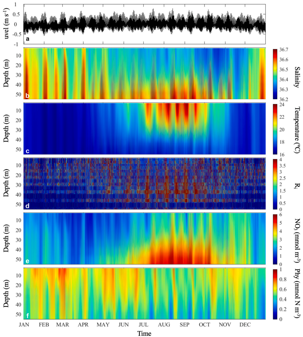
Fig. 8. (a) Temporal evolution of the mean zonal component of current velocity ( u_{vel} ; m s^{-1} ), computed for the whole water column at 6.11^{\circ}W and 36.06^{\circ}N (red circle in Fig. 1b), along the whole-year simulation. Hovmöller diagrams, computed at the same point (red circle in Fig. 1b), illustrating spatial (i.e., depth) and temporal variability of (b) salinity, (c) temperature ( ^{\circ}C ), (d) the Richardson number ( R_i , adimensional), (e) nitrate concentration ( NO_3 , mmol m^{-3} ) and (f) total phytoplankton biomass (Phy, mmol N m^{-3} ).
