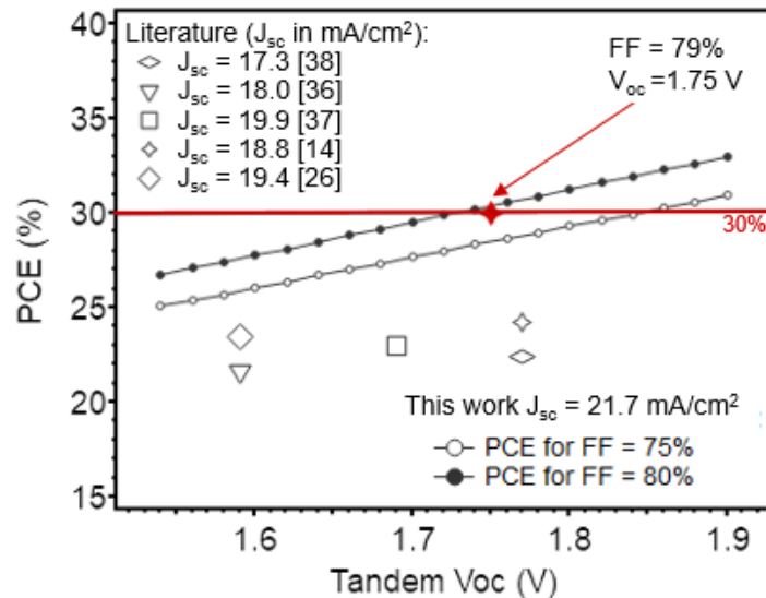
Figure 7 Predictions of the optimized tandem solar cell electrical performance, in comparison to the state-of-the-art certified literature devices. For this tandem structure (from this work), 30% efficiency is achievable for a V_{oc} of 1.75 V and a FF of 79% (red star). We point out that CI(G)S composition used in this work has a small bandgap (1.01 eV) which limits maximum attainable V_{oc} of the tandem, compared to the literature.
