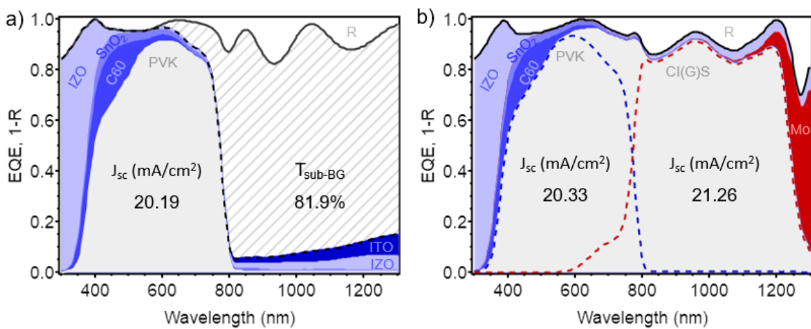
Figure 3 Optical loss analysis of the simulated structures, revealing sources of parasitic absorption in (a) semitransparent PVK solar cell, (b) PVK/CIS tandem solar cell.
