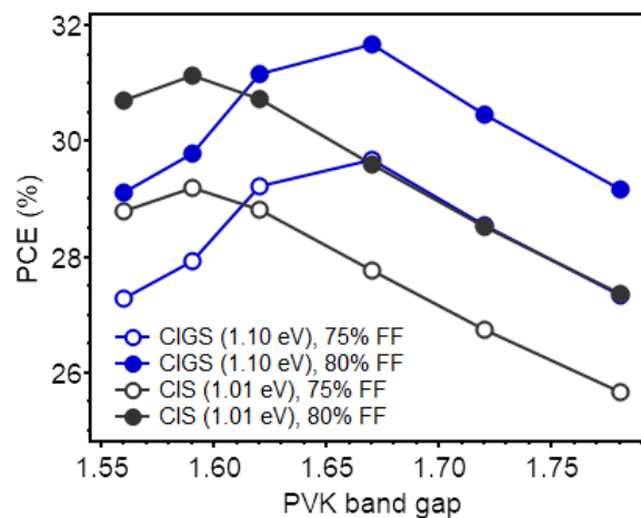
Figure 8 Power conversion efficiency (PCE) predictions for the structure from the paper with different perovskite bandgaps and with 2 different bottom cell bandgaps; CI(G)S ( E_g = 1.10 eV) in blue and CIS ( E_g = 1.01 eV) in black.
