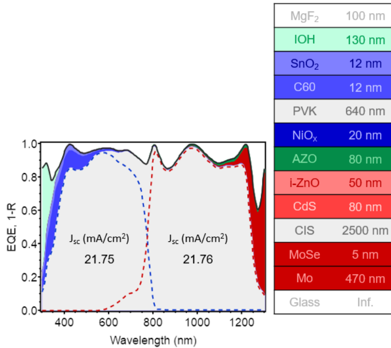
Figure 5 Optimized tandem solar cell from the Figure 1c. Decrease of parasitic absorption in UV-region (300-400 nm) has been achieved by applying changes from the semitransparent perovskite solar cell optimization. Current matching was achieved by adjusting thicknesses of other layers, mainly AZO and PVK.
