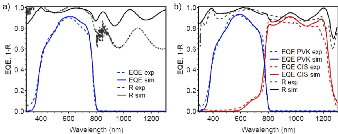
Figure 2 Comparison of the simulated reflectance and EQE with the experimental results for (a) the semitransparent PVK solar cell; (b) the PVK/CIS tandem. Solid lines represent the simulated curves, while the dashed lines represent the experimental data.
