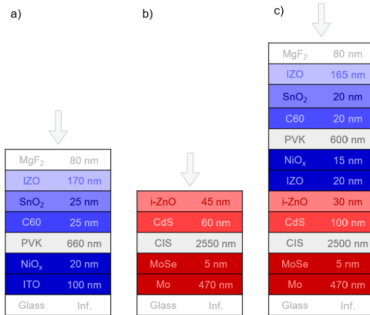
Figure 1 Simulated optical structures: (a) semitransparent PVK single junction solar cell; (b) CIS substrate and (c) PVK/CIS 2T tandem [as in 26]. The arrows indicate the illumination direction.
