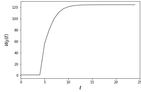
Figure 2: W_\beta(\ell) as a function of \ell with \beta = 5 and parameters f = 0.03 , \delta = 0.1 , \epsilon = 10^{-5} , and \lambda = 1,000 .
