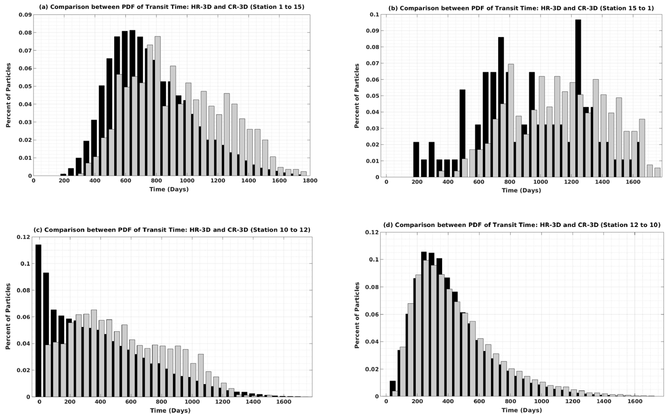
Figure 5. Comparison of HR-3D (black) and CR-3D (gray) transit time distributions (a) for particles initially deployed from site 1 to site 15, (b) from site 15 to site 1, (c) from site 10 to site 12, and (d) from site 12 to site 10.
