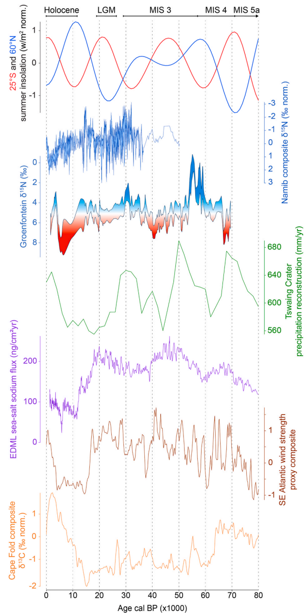
Fig. 6. Comparison of the \delta^{15}\text{N} data from the Groenfontein-1 rock hyrax midden (shading: blue (red) = wetter (drier) than average conditions) with: summer insolation at 25°S and 60°N (Laskar et al., 2004), a composite \delta^{15}\text{N} record from the Namib Desert region (Chase et al., 2019b), the precipitation reconstruction from Tswaing Crater (Partridge et al., 1997), the sea-salt sodium flux record from the Dronning Maud Land (EDML) Antarctic ice core (Fischer et al., 2007), a composite record of SE Atlantic wind strength proxies (higher values indicate increased wind strength; Chase et al., 2019a; data from Farmer et al., 2005; Little et al., 1997; Pichevin et al., 2005; Stuut et al., 2002), and the Cape Fold composite \delta^{13}\text{C} record (Chase et al., 2021; including data from Braun et al., 2020; Chase et al., 2017; Talma and Vogel, 1992). (For interpretation of the references to colour in this figure legend, the reader is referred to the Web version of this article.)
