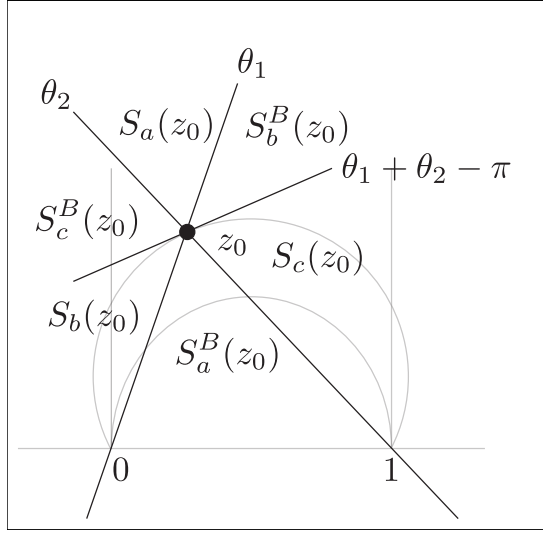
FIGURE 4. The decomposition of the tangent space at z_0 into six sectors
