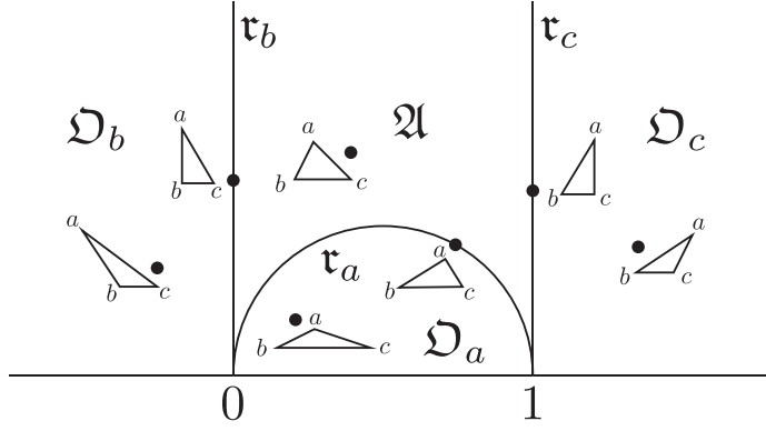
FIGURE 1. The space of triangles \mathfrak{T}_A . The hyperbolic ideal triangle \mathfrak{A} with vertex \{0, 1, \infty\} is identified with the space \mathfrak{AT}_A of acute triangles. For v \in \{a, b, c\} , \mathfrak{r}_v consists of right triangles whose angle is \pi/2 at the v -vertex, and \mathfrak{D}_v consists of obtuse triangles which have an obtuse angle at the vertex labelled v .
