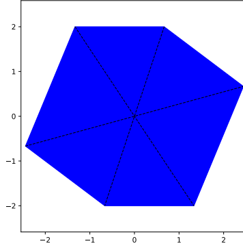
FIGURE 5. The shape of the Finsler unit ball at z_0 = 1/3 + i . The diagonals (dashed lines) divide the hexagon into six triangles and each triangle is similar to T_{z_0} .
