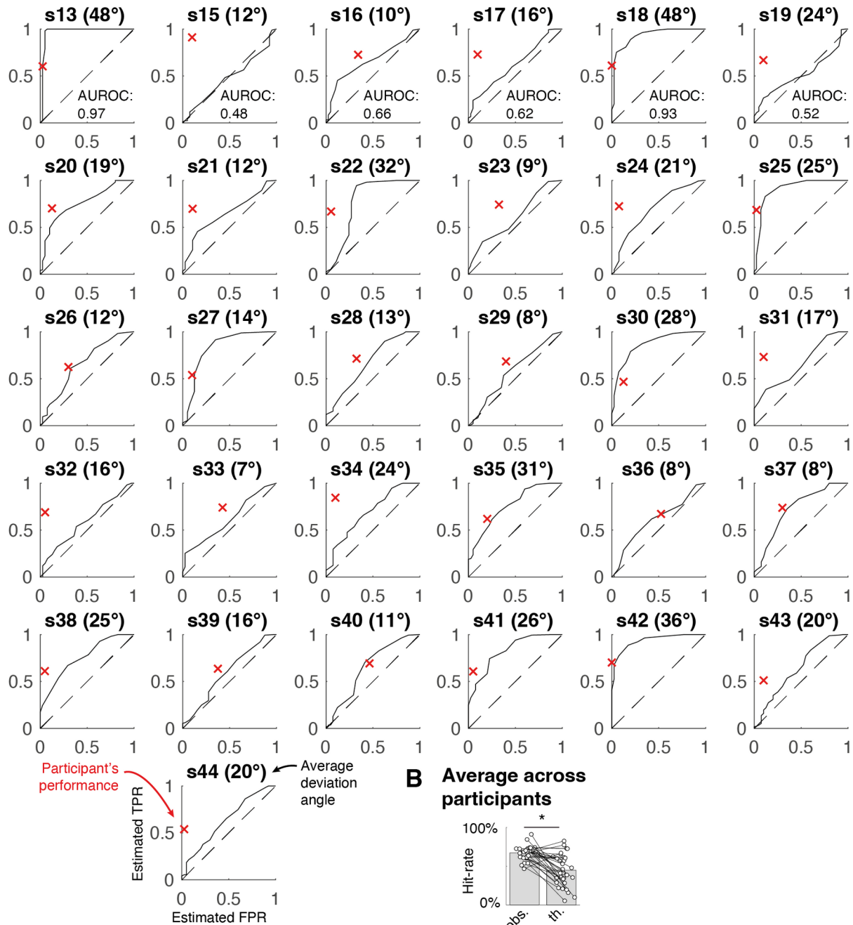
702 Figure 1 - 4 703 Receiving operating curve (ROC) analysis for detection.
