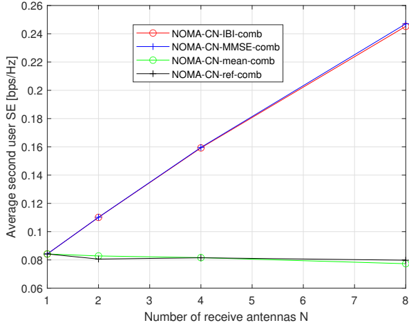
Fig. 7: Average spectral efficiency of second users vs. the number of receive antennas N , for multi-antenna receivers
