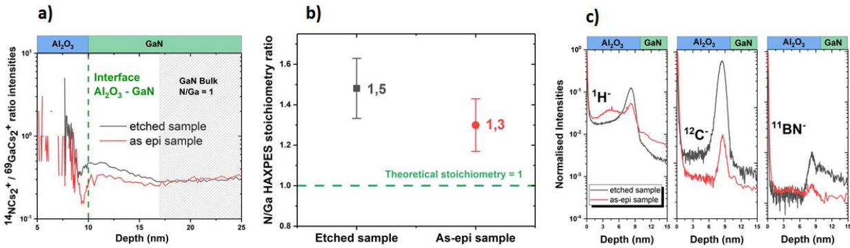
Figure 3: (a) ^{14}\text{N/Cs}_2^+ / ^{69}\text{Ga/Cs}_2^+ ratio depth profile (b) N/Ga HAXPES stoichiometry of core level spectrum N 1s/Ga 2p 3/2 and (c) ToF-SIMS depth profiles of etched and as-epi samples of the main impurities present at the Al 2 O 3 /GaN interface.
