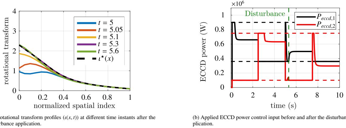
Fig. 12: t -profiles and applied ECCD power ( P_{ECCD,i} ) for the two antennas in case the point to be regulated is different from the one the controller has been trained with and external disturbance application.
