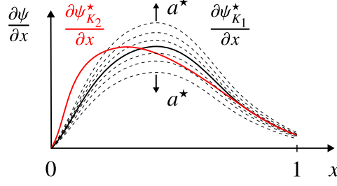
Fig. 2: Examples of different poloidal magnetic flux equilibriums of the reaction-diffusion equation describing the magnetic flux dynamics. In black we show that with a certain set of parameters K_1 , changing the applied constant input (ECCD power), the poloidal magnetic flux equilibrium changes. The red profile represent a possible poloidal magnetic flux equilibrium with a different set of parameters K_2 .
