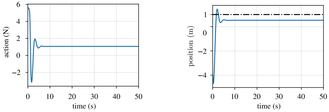
Fig. C.15: Control action and position of the mass-spring damper system in closed loop with a controller without integral state that has been trained on a model with a different spring coefficient.
